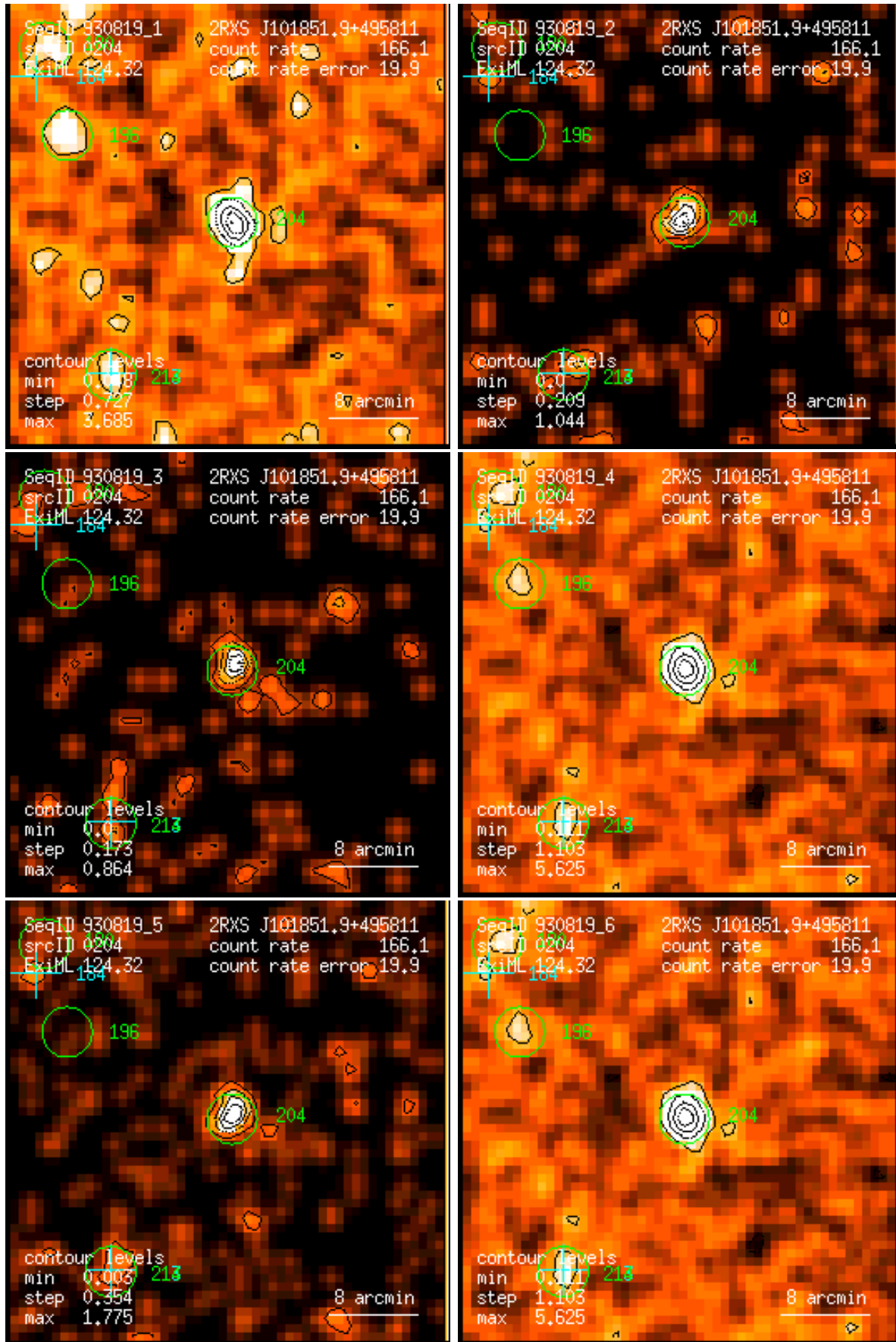
Figure 204: RASS 930819: detection 0204: band rate images, Gaussian filter: (1) PSPC channels 11 – 41, (2) 52 – 90, (3) 91 – 201, (4) 11 – 235, (5) 52 – 201, (6) 11 – 201. Broad band rates in counts/ks. Band rate contour levels in counts/ks/arcmin 2 .
