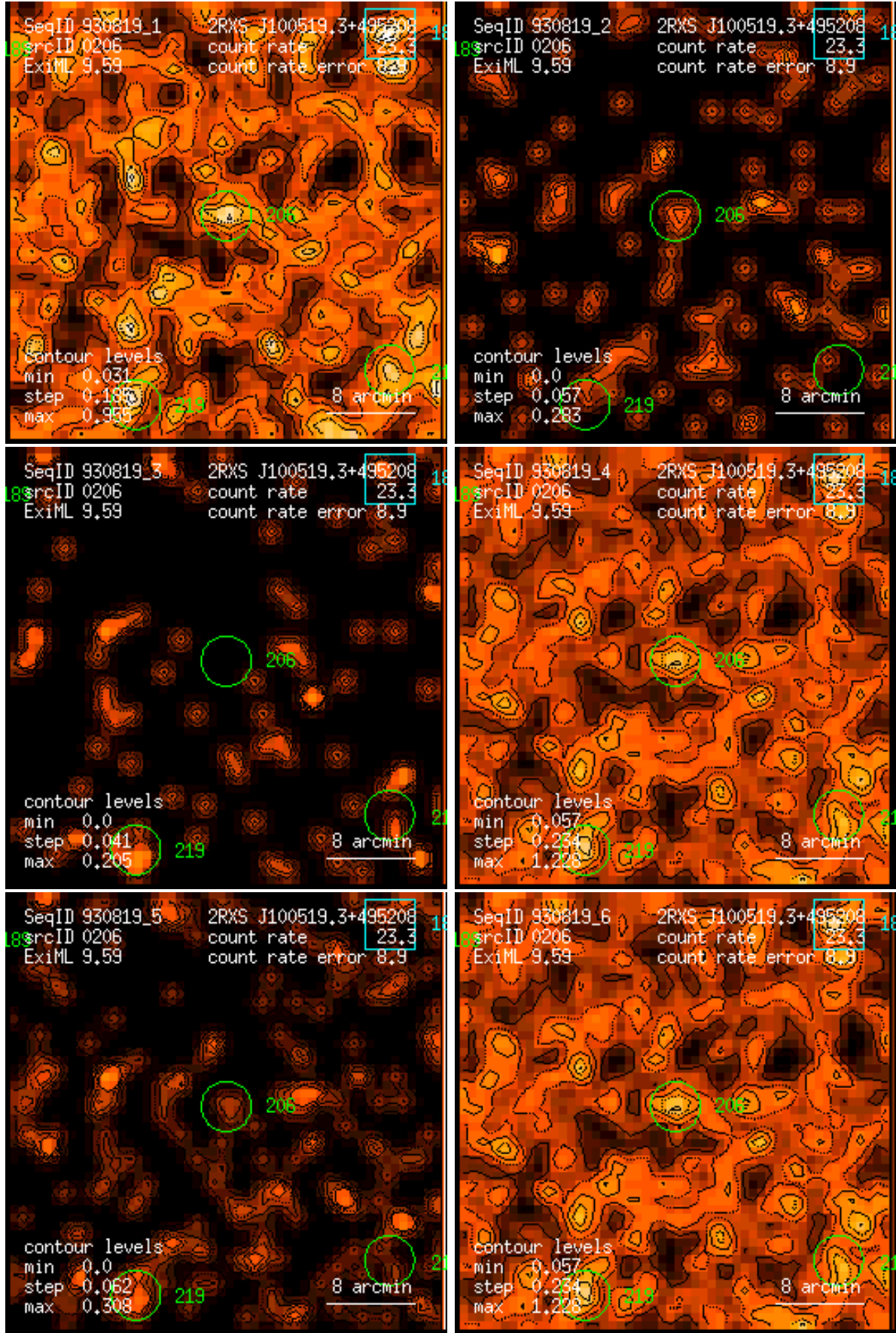
Figure 206: RASS 930819: detection 0206: band rate images, Gaussian filter: (1) PSPC channels 11 – 41, (2) 52 – 90, (3) 91 – 201, (4) 11 – 235, (5) 52 – 201, (6) 11 – 201. Broad band rates in counts/ks. Band rate contour levels in counts/ks/arcmin 2 .
