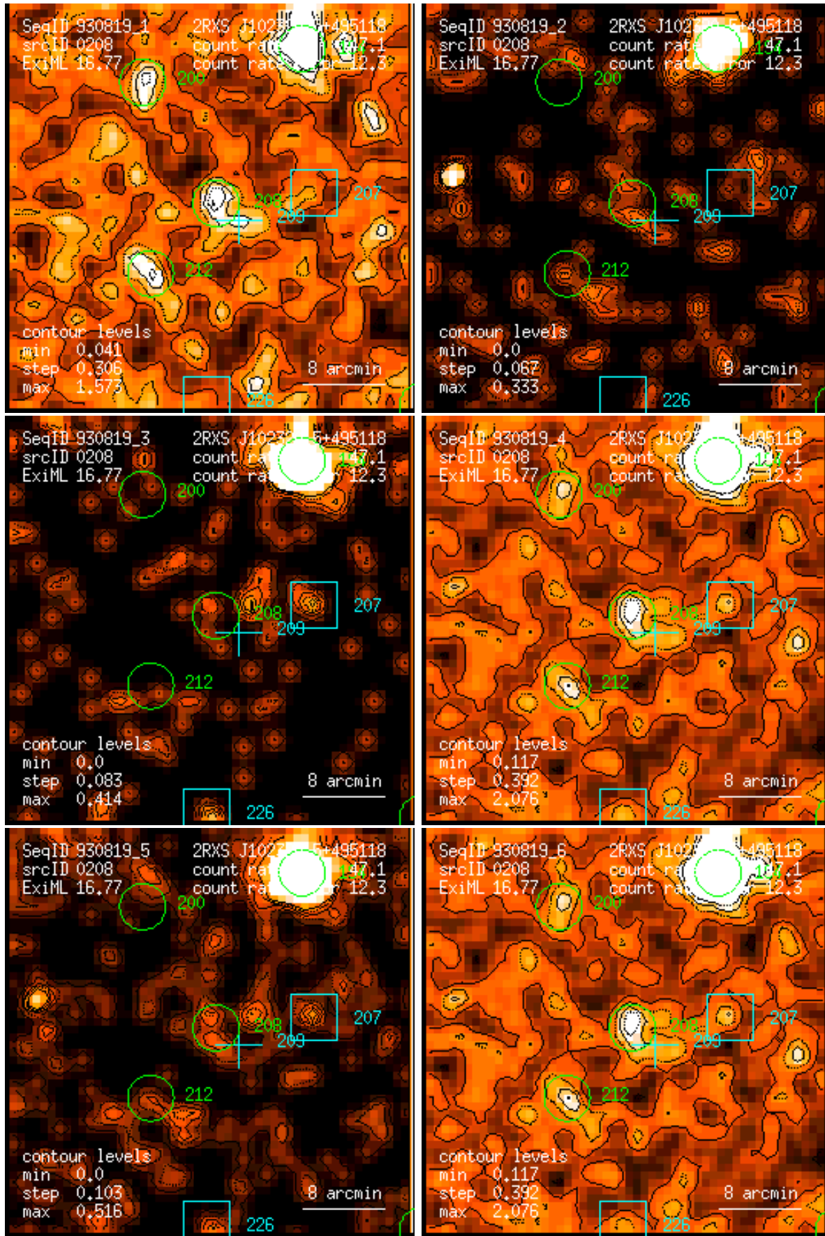
Figure 208: RASS 930819: detection 0208: band rate images, Gaussian filter: (1) PSPC channels 11 – 41, (2) 52 – 90, (3) 91 – 201, (4) 11 – 235, (5) 52 – 201, (6) 11 – 201. Broad band rates in counts/ks. Band rate contour levels in counts/ks/arcmin 2 .
