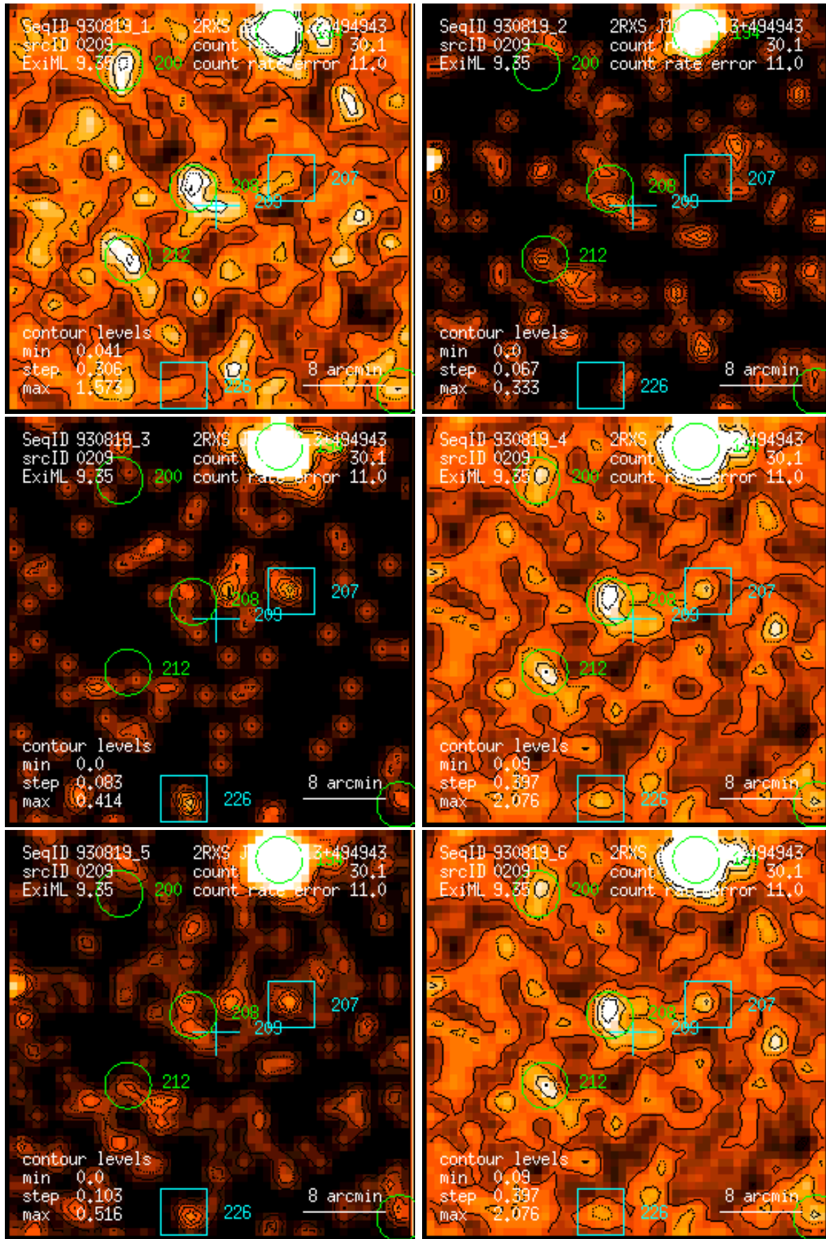
Figure 209: RASS 930819: detection 0209: band rate images, Gaussian filter: (1) PSPC channels 11 – 41, (2) 52 – 90, (3) 91 – 201, (4) 11 – 235, (5) 52 – 201, (6) 11 – 201. Broad band rates in counts/ks. Band rate contour levels in counts/ks/arcmin 2 .
