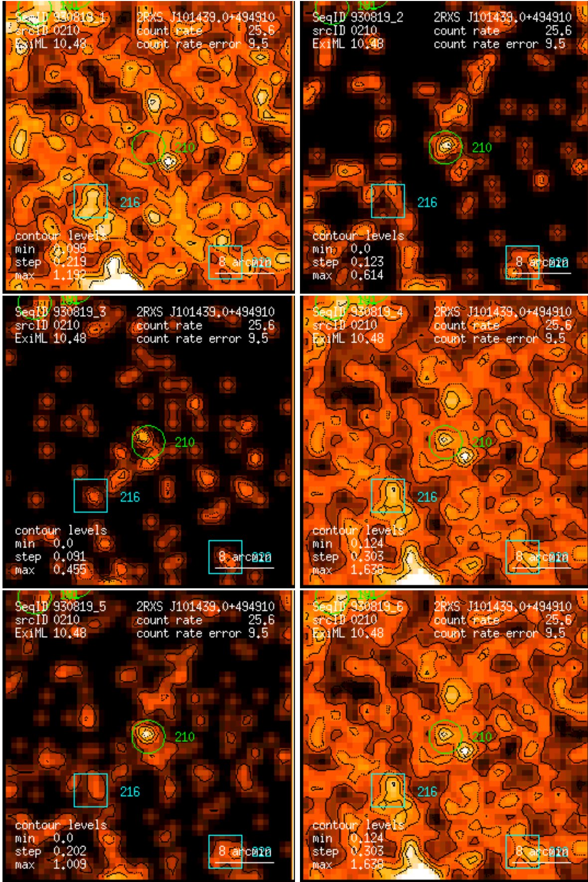
Figure 210: RASS 930819: detection 0210: band rate images, Gaussian filter: (1) PSPC channels 11 – 41, (2) 52 – 90, (3) 91 – 201, (4) 11 – 235, (5) 52 – 201, (6) 11 – 201. Broad band rates in counts/ks. Band rate contour levels in counts/ks/arcmin 2 .
