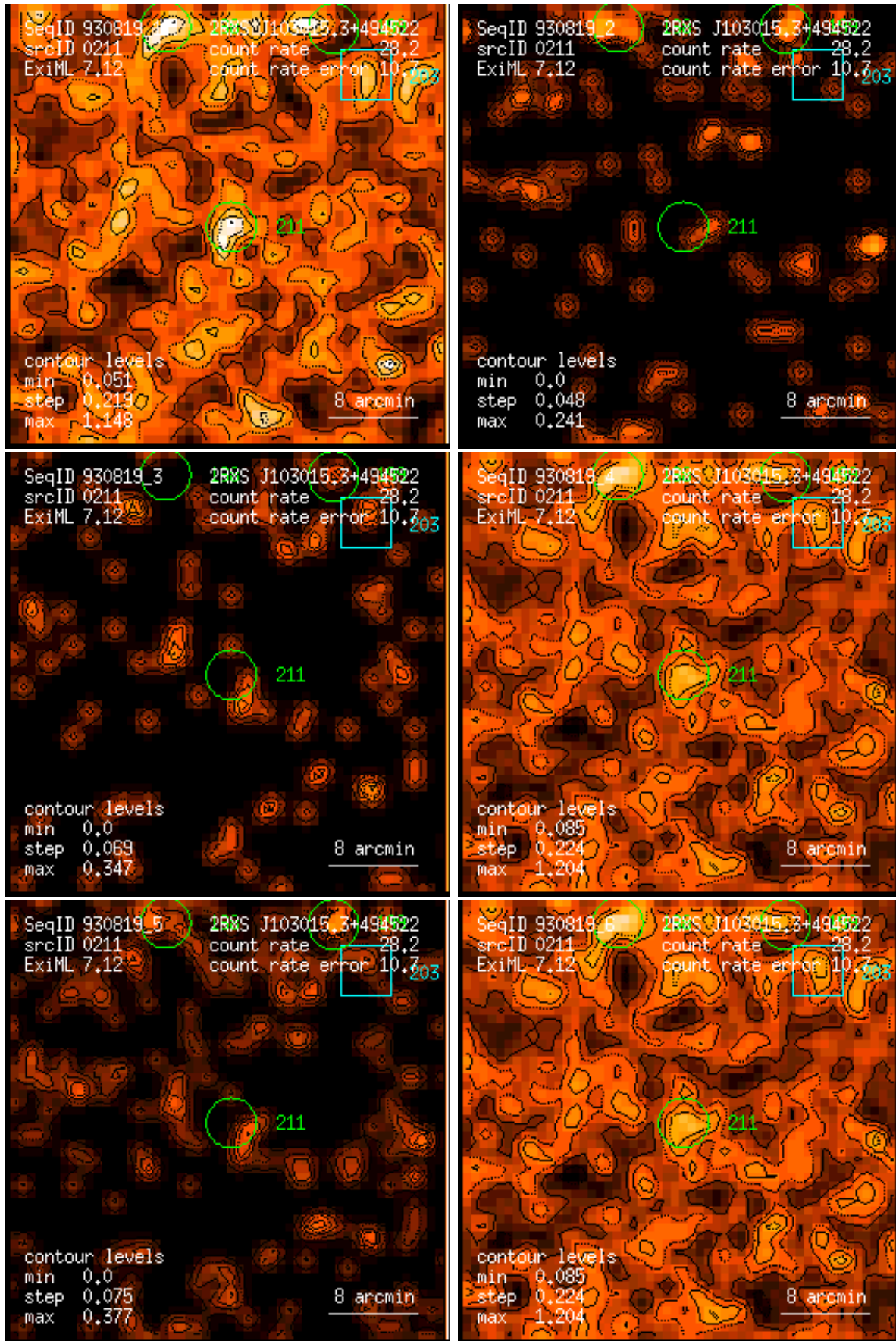
Figure 211: RASS 930819: detection 0211: band rate images, Gaussian filter: (1) PSPC channels 11 – 41, (2) 52 – 90, (3) 91 – 201, (4) 11 – 235, (5) 52 – 201, (6) 11 – 201. Broad band rates in counts/ks. Band rate contour levels in counts/ks/arcmin 2 .
