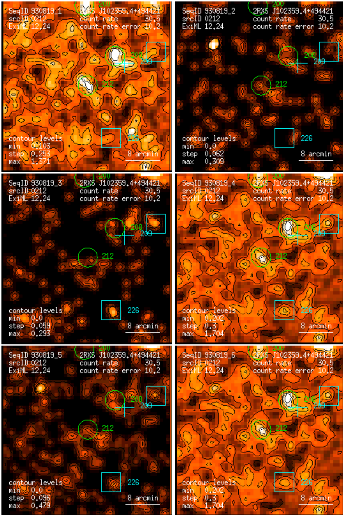
Figure 212: RASS 930819: detection 0212: band rate images, Gaussian filter: (1) PSPC channels 11 – 41, (2) 52 – 90, (3) 91 – 201, (4) 11 – 235, (5) 52 – 201, (6) 11 – 201. Broad band rates in counts/ks. Band rate contour levels in counts/ks/arcmin 2 .
