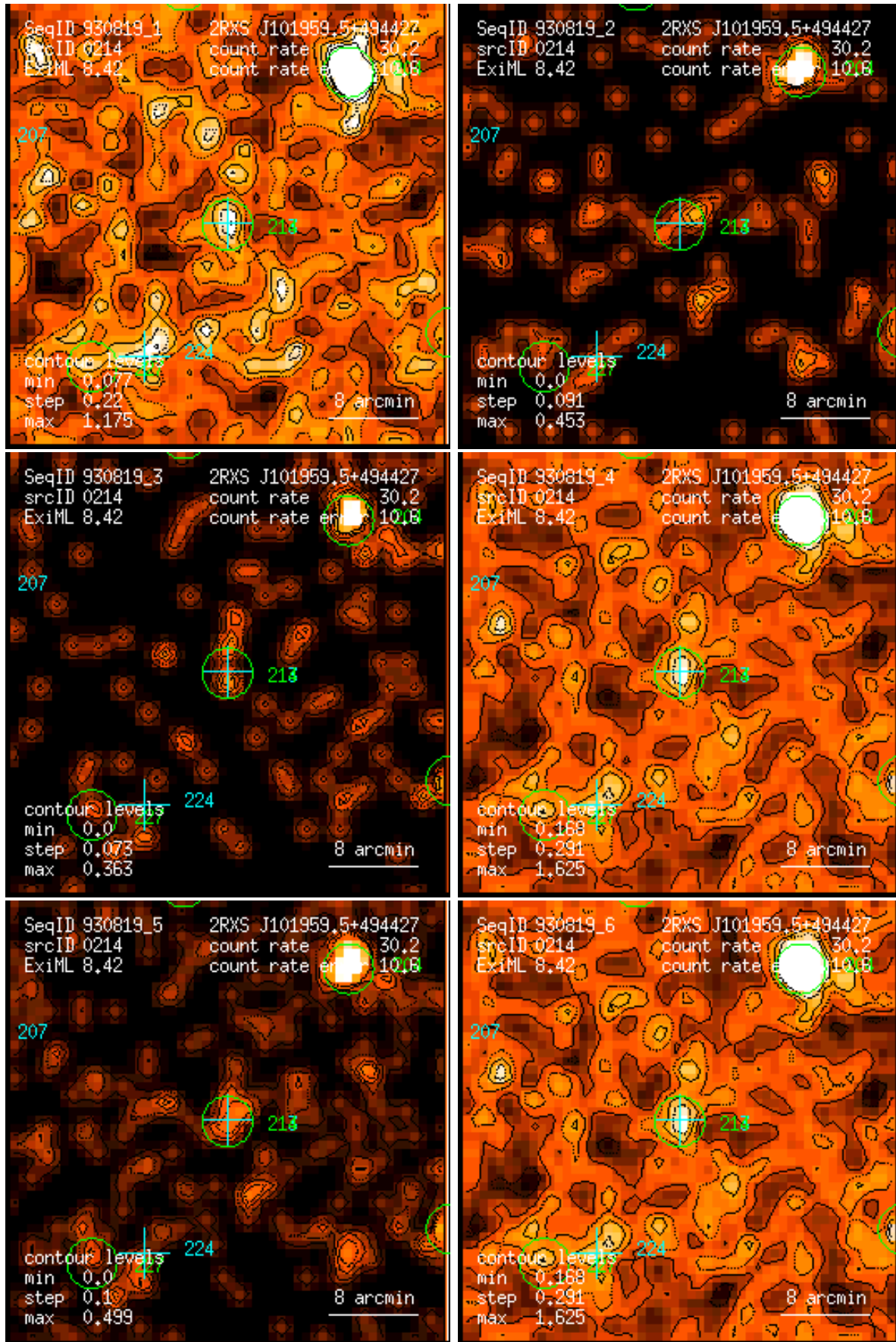
Figure 214: RASS 930819: detection 0214: band rate images, Gaussian filter: (1) PSPC channels 11 – 41, (2) 52 – 90, (3) 91 – 201, (4) 11 – 235, (5) 52 – 201, (6) 11 – 201. Broad band rates in counts/ks. Band rate contour levels in counts/ks/arcmin 2 .
