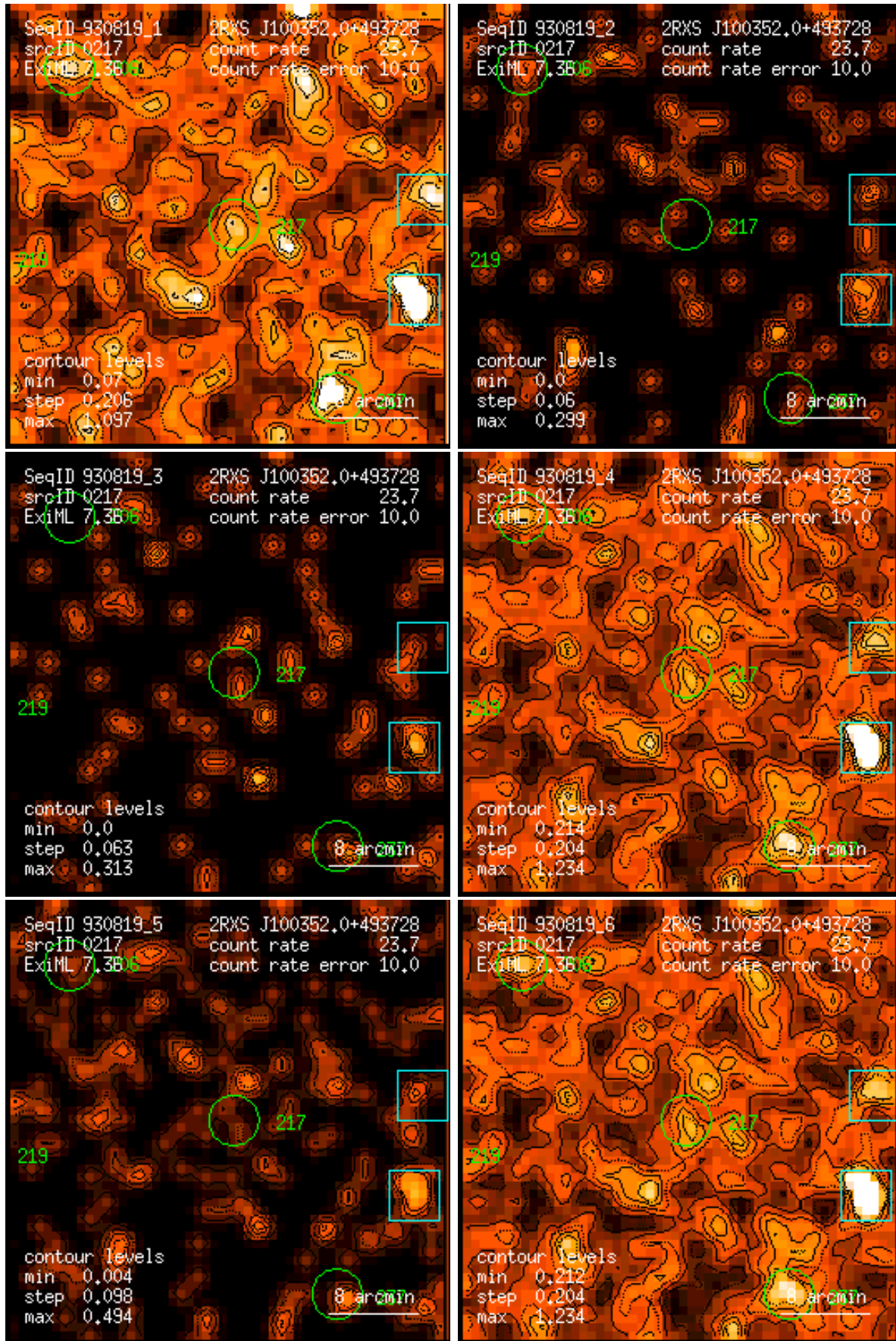
Figure 217: RASS 930819: detection 0217: band rate images, Gaussian filter: (1) PSPC channels 11 – 41, (2) 52 – 90, (3) 91 – 201, (4) 11 – 235, (5) 52 – 201, (6) 11 – 201. Broad band rates in counts/ks. Band rate contour levels in counts/ks/arcmin 2 .
