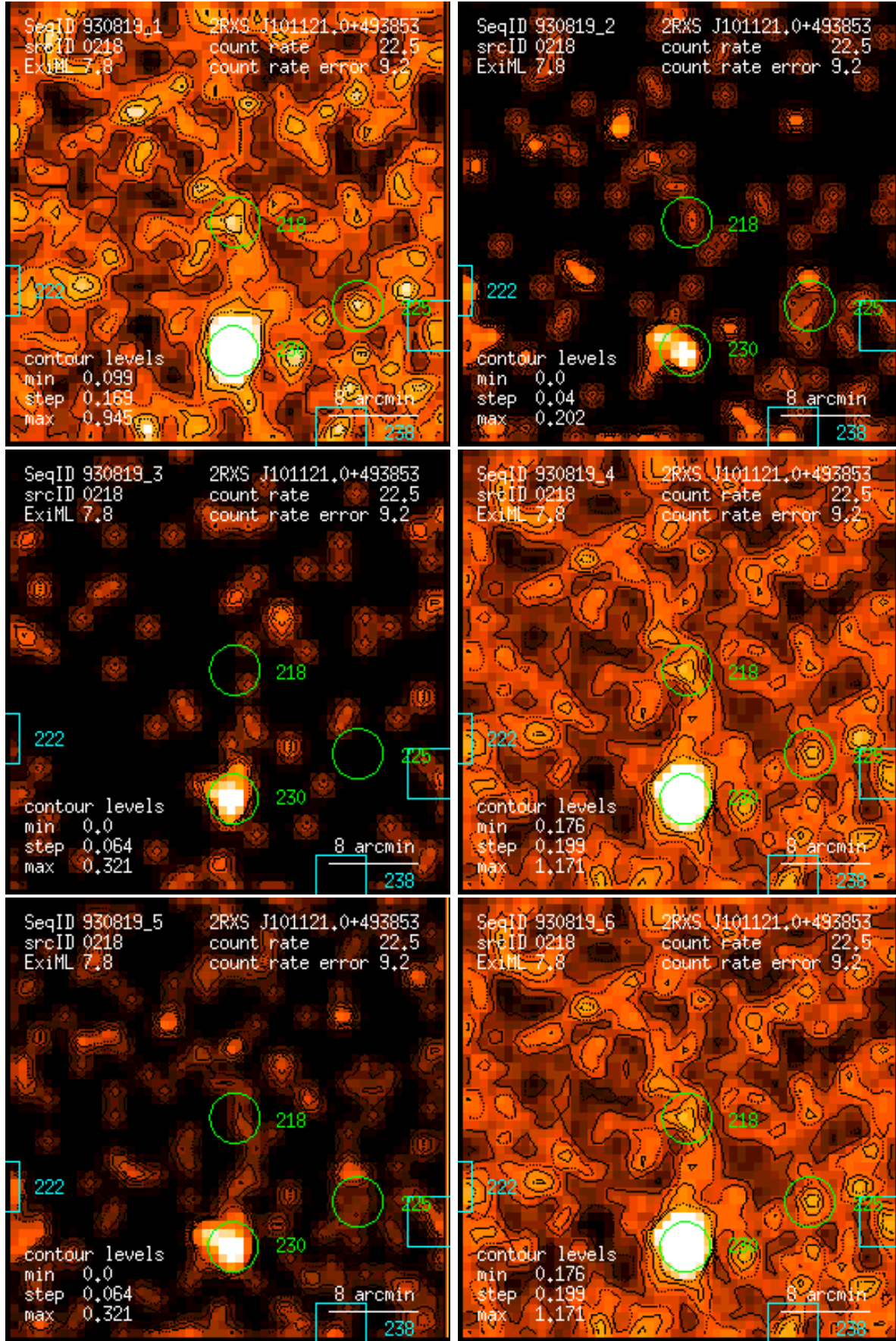
Figure 218: RASS 930819: detection 0218: band rate images, Gaussian filter: (1) PSPC channels 11 – 41, (2) 52 – 90, (3) 91 – 201, (4) 11 – 235, (5) 52 – 201, (6) 11 – 201. Broad band rates in counts/ks. Band rate contour levels in counts/ks/arcmin 2 .
