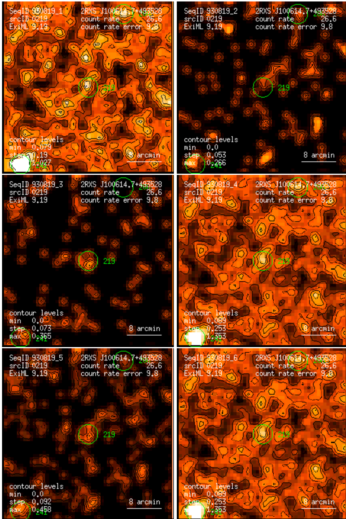
Figure 219: RASS 930819: detection 0219: band rate images, Gaussian filter: (1) PSPC channels 11 – 41, (2) 52 – 90, (3) 91 – 201, (4) 11 – 235, (5) 52 – 201, (6) 11 – 201. Broad band rates in counts/ks. Band rate contour levels in counts/ks/arcmin 2 .
