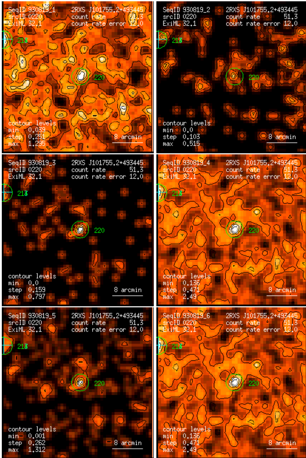
Figure 220: RASS 930819: detection 0220: band rate images, Gaussian filter: (1) PSPC channels 11 – 41, (2) 52 – 90, (3) 91 – 201, (4) 11 – 235, (5) 52 – 201, (6) 11 – 201. Broad band rates in counts/ks. Band rate contour levels in counts/ks/arcmin 2 .
