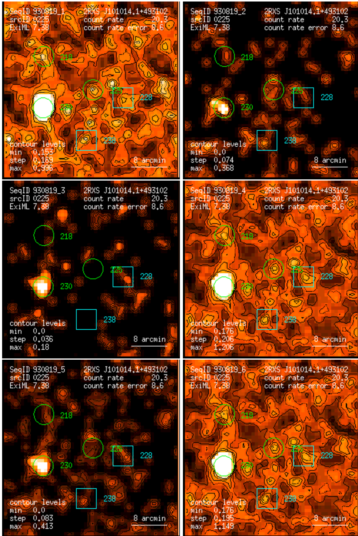
Figure 225: RASS 930819: detection 0225: band rate images, Gaussian filter: (1) PSPC channels 11 – 41, (2) 52 – 90, (3) 91 – 201, (4) 11 – 235, (5) 52 – 201, (6) 11 – 201. Broad band rates in counts/ks. Band rate contour levels in counts/ks/arcmin 2 .
