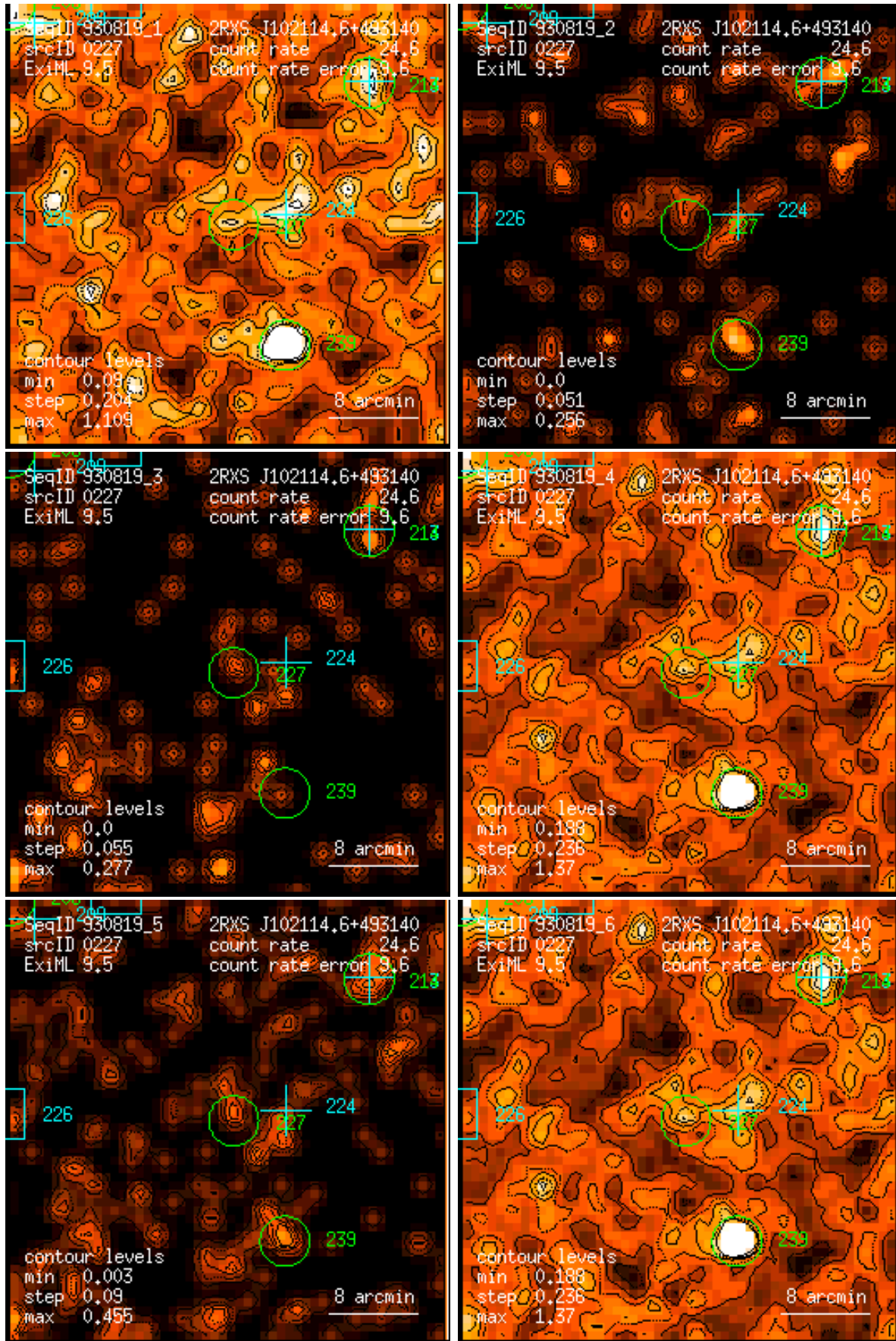
Figure 227: RASS 930819: detection 0227: band rate images, Gaussian filter: (1) PSPC channels 11 – 41, (2) 52 – 90, (3) 91 – 201, (4) 11 – 235, (5) 52 – 201, (6) 11 – 201. Broad band rates in counts/ks. Band rate contour levels in counts/ks/arcmin 2 .
