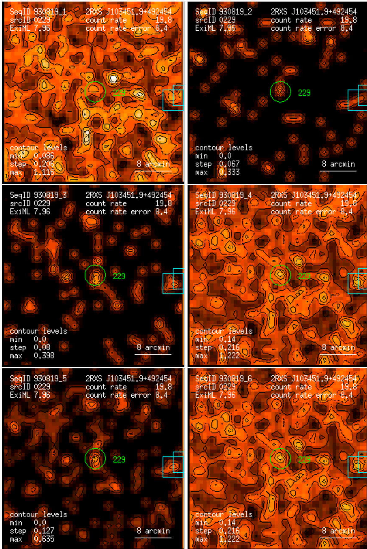
Figure 229: RASS 930819: detection 0229: band rate images, Gaussian filter: (1) PSPC channels 11 – 41, (2) 52 – 90, (3) 91 – 201, (4) 11 – 235, (5) 52 – 201, (6) 11 – 201. Broad band rates in counts/ks. Band rate contour levels in counts/ks/arcmin 2 .
