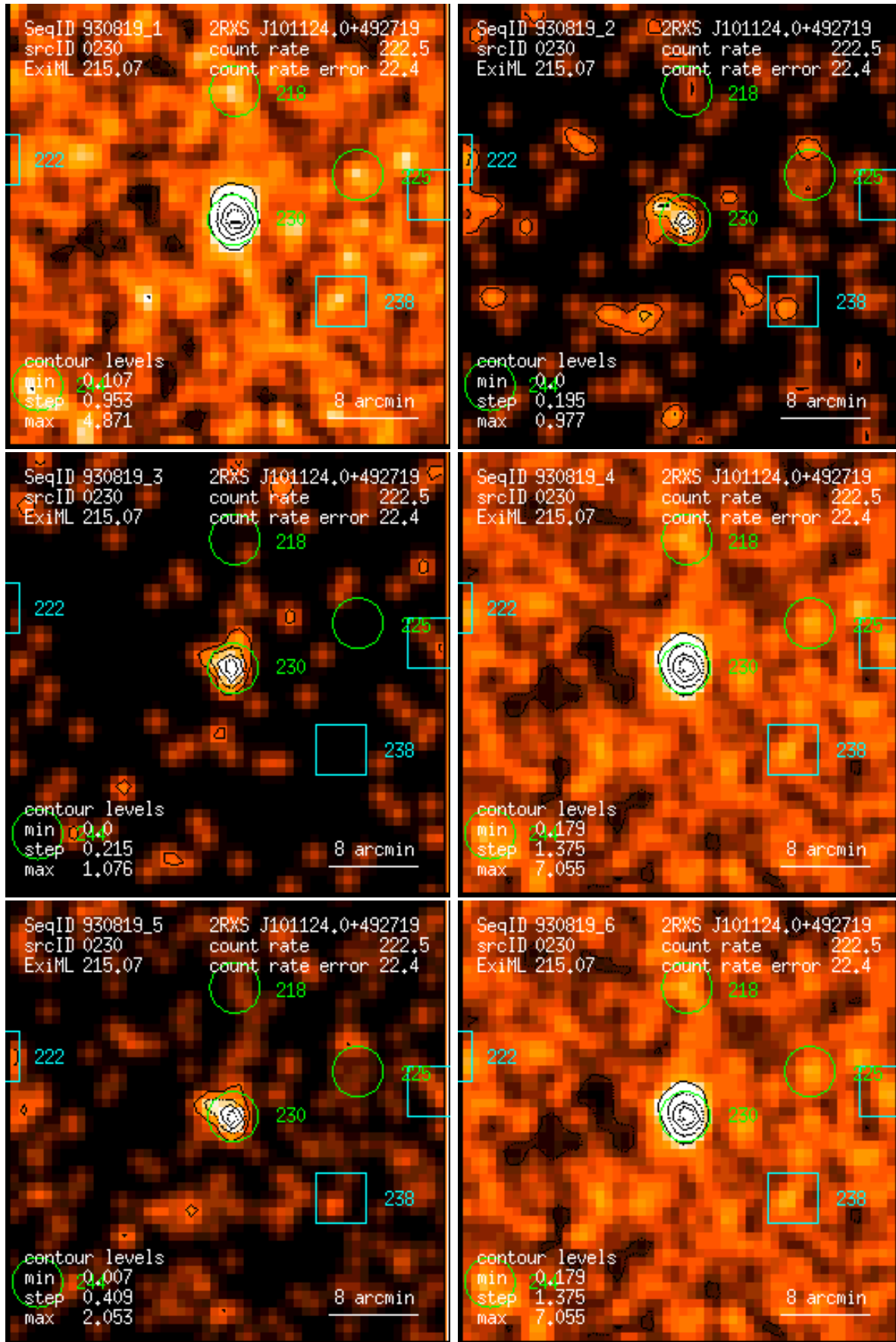
Figure 230: RASS 930819: detection 0230: band rate images, Gaussian filter: (1) PSPC channels 11 – 41, (2) 52 – 90, (3) 91 – 201, (4) 11 – 235, (5) 52 – 201, (6) 11 – 201. Broad band rates in counts/ks. Band rate contour levels in counts/ks/arcmin 2 .
