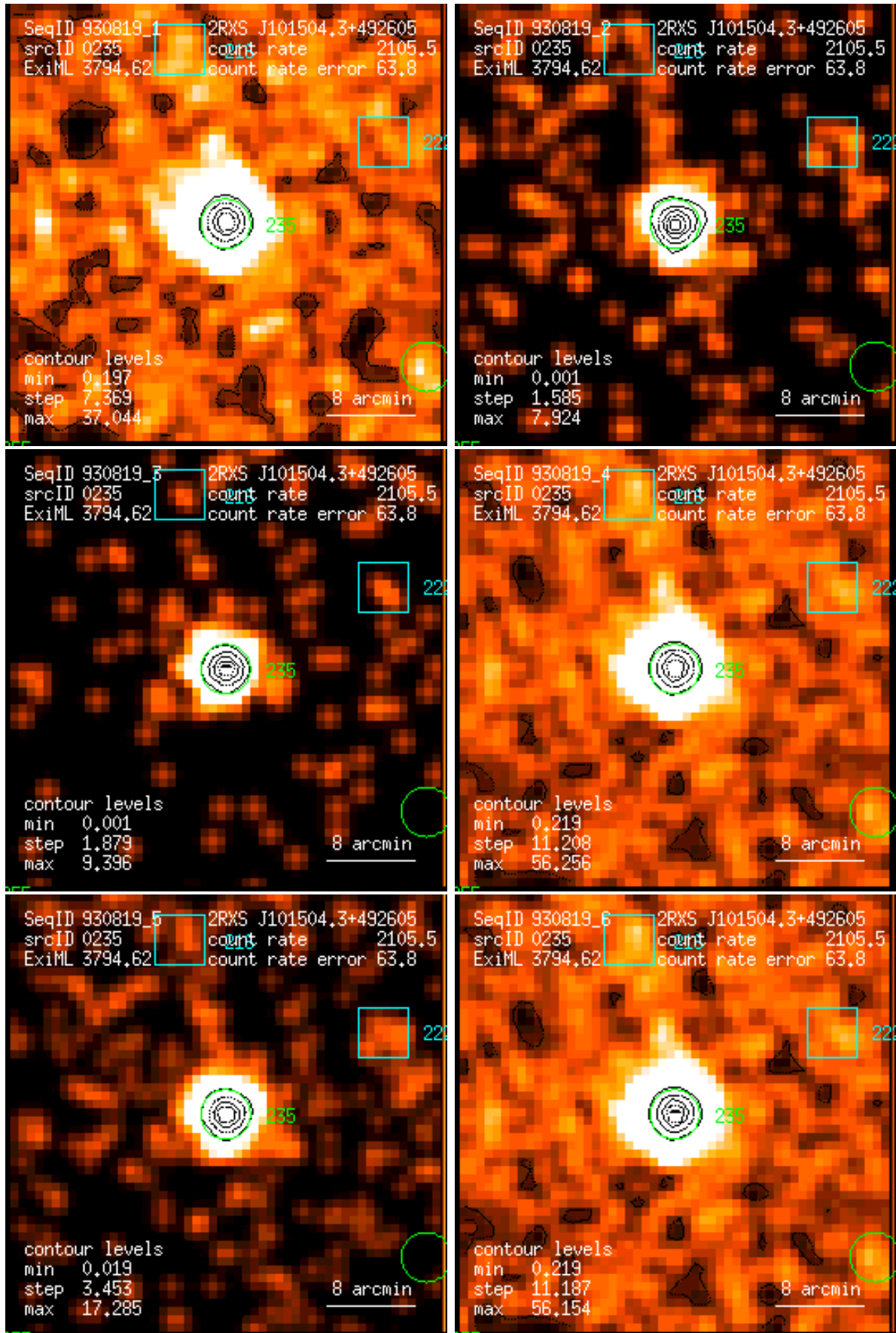
Figure 235: RASS 930819: detection 0235: band rate images, Gaussian filter: (1) PSPC channels 11 – 41, (2) 52 – 90, (3) 91 – 201, (4) 11 – 235, (5) 52 – 201, (6) 11 – 201. Broad band rates in counts/ks. Band rate contour levels in counts/ks/arcmin 2 .
