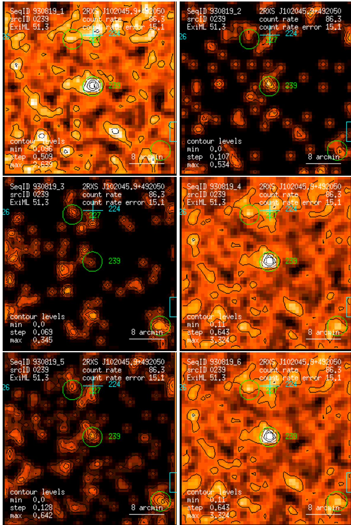
Figure 239: RASS 930819: detection 0239: band rate images, Gaussian filter: (1) PSPC channels 11 – 41, (2) 52 – 90, (3) 91 – 201, (4) 11 – 235, (5) 52 – 201, (6) 11 – 201. Broad band rates in counts/ks. Band rate contour levels in counts/ks/arcmin 2 .
