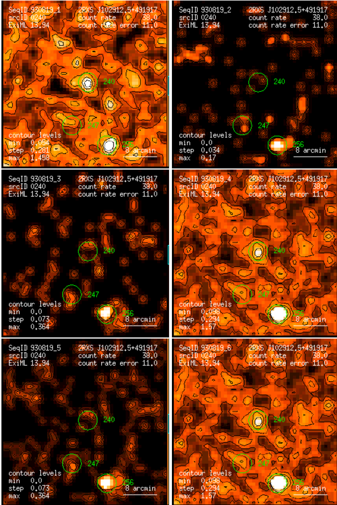
Figure 240: RASS 930819: detection 0240: band rate images, Gaussian filter: (1) PSPC channels 11 – 41, (2) 52 – 90, (3) 91 – 201, (4) 11 – 235, (5) 52 – 201, (6) 11 – 201. Broad band rates in counts/ks. Band rate contour levels in counts/ks/arcmin 2 .
