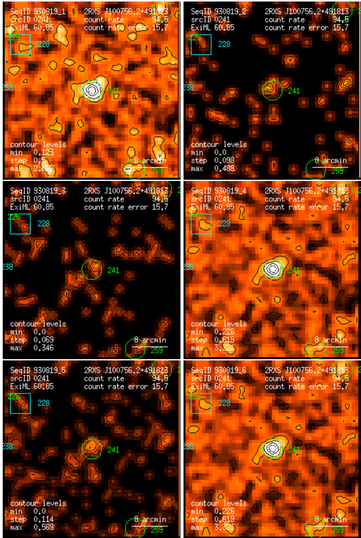
Figure 241: RASS 930819: detection 0241: band rate images, Gaussian filter: (1) PSPC channels 11 – 41, (2) 52 – 90, (3) 91 – 201, (4) 11 – 235, (5) 52 – 201, (6) 11 – 201. Broad band rates in counts/ks. Band rate contour levels in counts/ks/arcmin 2 .
