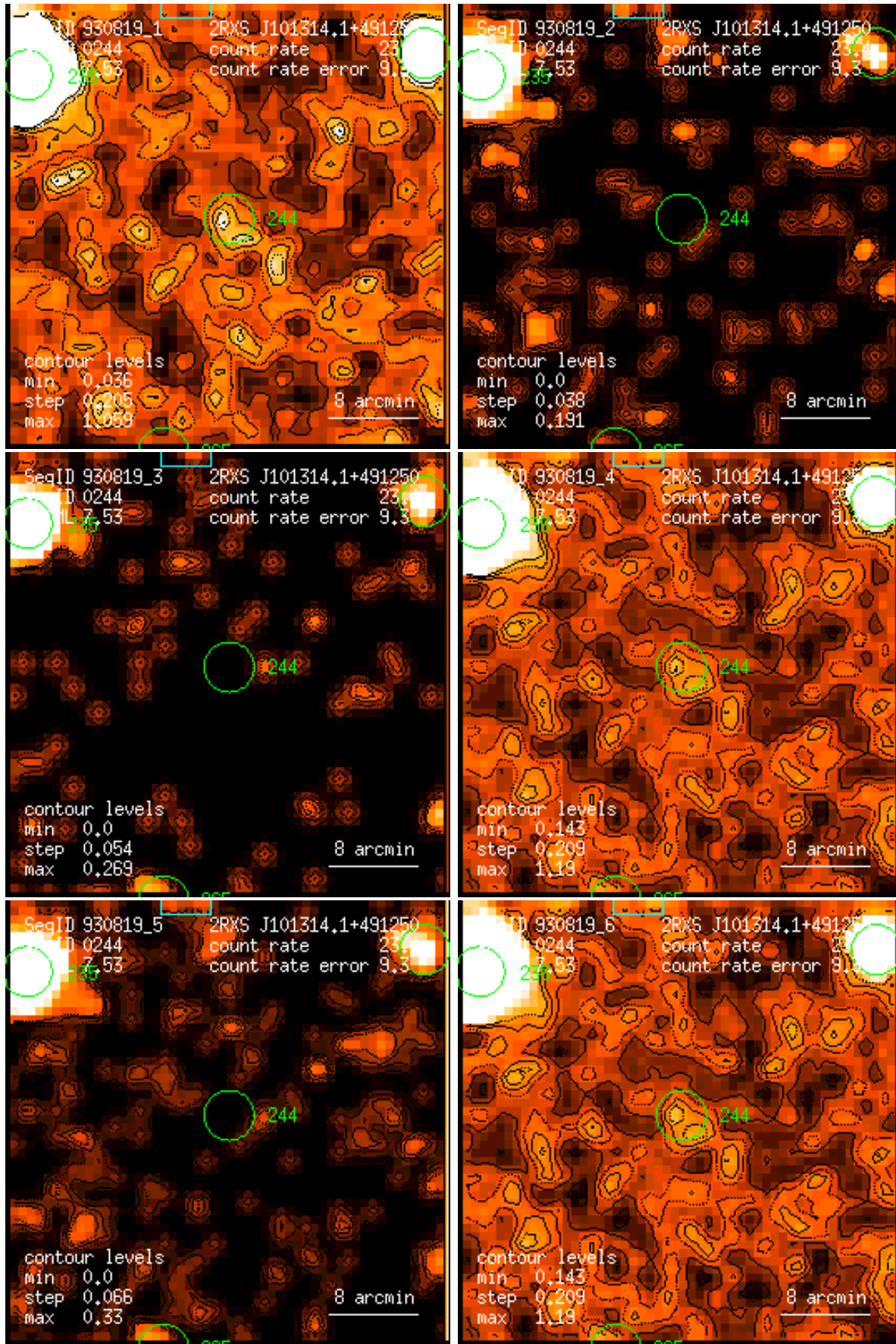
Figure 244: RASS 930819: detection 0244: band rate images, Gaussian filter: (1) PSPC channels 11 – 41, (2) 52 – 90, (3) 91 – 201, (4) 11 – 235, (5) 52 – 201, (6) 11 – 201. Broad band rates in counts/ks. Band rate contour levels in counts/ks/arcmin 2 .
