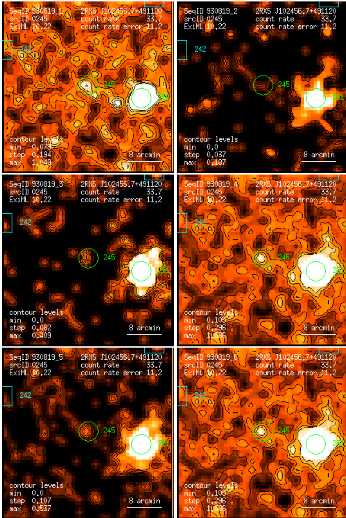
Figure 245: RASS 930819: detection 0245: band rate images, Gaussian filter: (1) PSPC channels 11 – 41, (2) 52 – 90, (3) 91 – 201, (4) 11 – 235, (5) 52 – 201, (6) 11 – 201. Broad band rates in counts/ks. Band rate contour levels in counts/ks/arcmin 2 .
