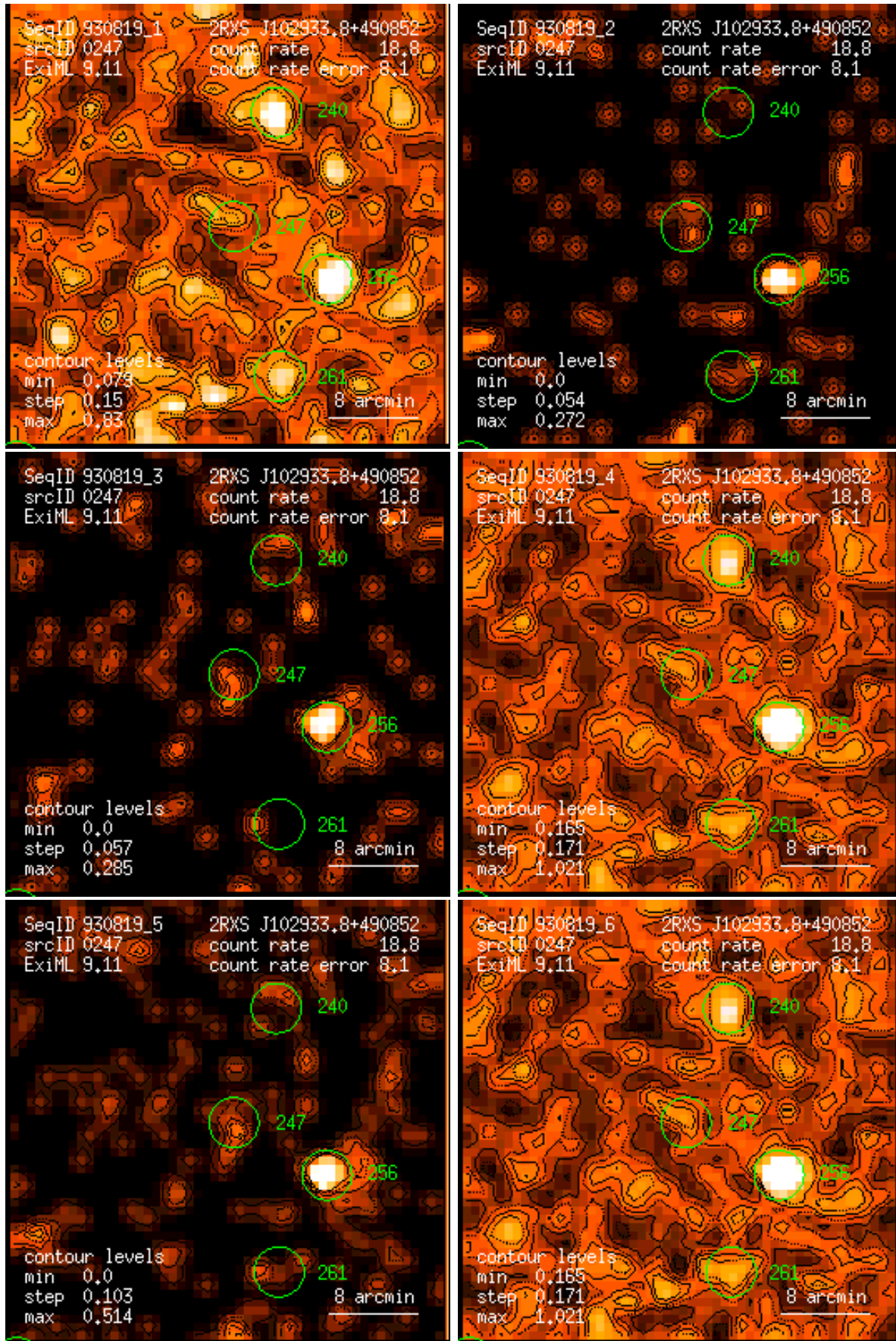
Figure 247: RASS 930819: detection 0247: band rate images, Gaussian filter: (1) PSPC channels 11 – 41, (2) 52 – 90, (3) 91 – 201, (4) 11 – 235, (5) 52 – 201, (6) 11 – 201. Broad band rates in counts/ks. Band rate contour levels in counts/ks/arcmin 2 .
