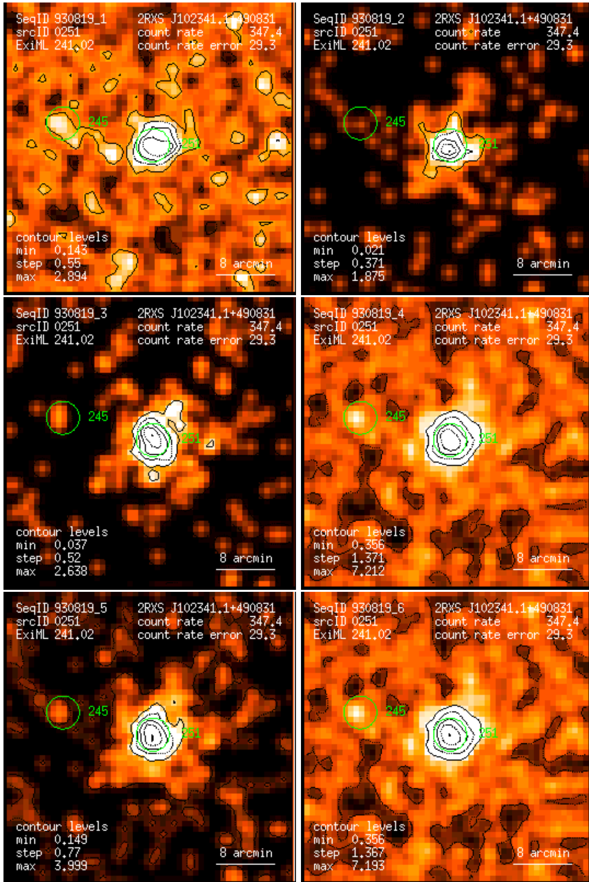
Figure 251: RASS 930819: detection 0251: band rate images, Gaussian filter: (1) PSPC channels 11 – 41, (2) 52 – 90, (3) 91 – 201, (4) 11 – 235, (5) 52 – 201, (6) 11 – 201. Broad band rates in counts/ks. Band rate contour levels in counts/ks/arcmin 2 .
