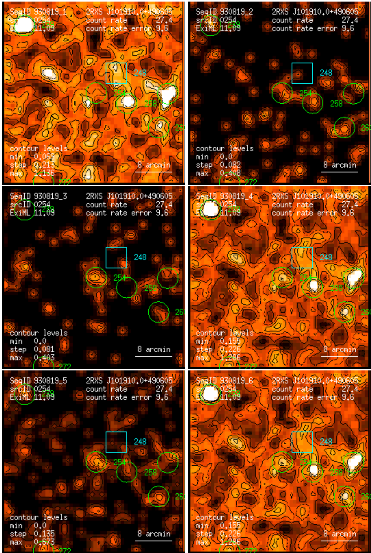
Figure 254: RASS 930819: detection 0254: band rate images, Gaussian filter: (1) PSPC channels 11 – 41, (2) 52 – 90, (3) 91 – 201, (4) 11 – 235, (5) 52 – 201, (6) 11 – 201. Broad band rates in counts/ks. Band rate contour levels in counts/ks/arcmin 2 .
