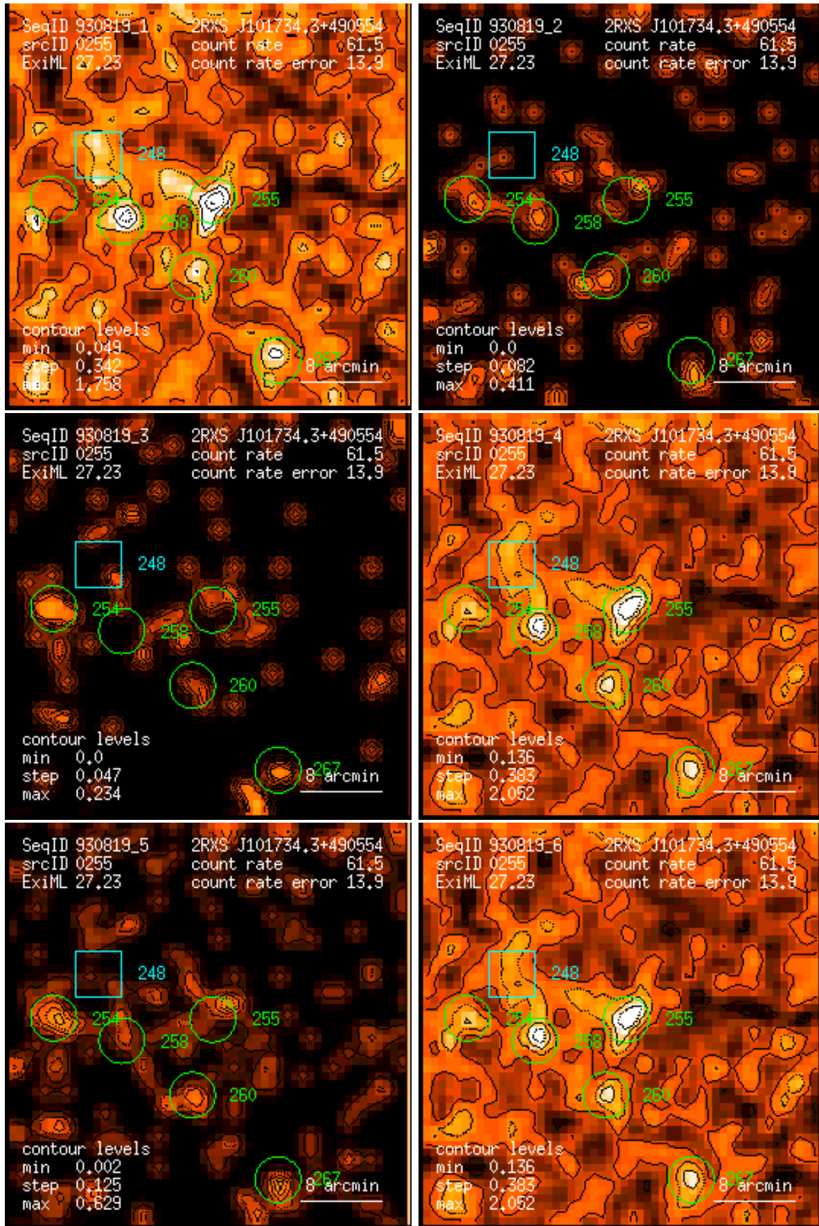
Figure 255: RASS 930819: detection 0255: band rate images, Gaussian filter: (1) PSPC channels 11 – 41, (2) 52 – 90, (3) 91 – 201, (4) 11 – 235, (5) 52 – 201, (6) 11 – 201. Broad band rates in counts/ks. Band rate contour levels in counts/ks/arcmin 2 .
