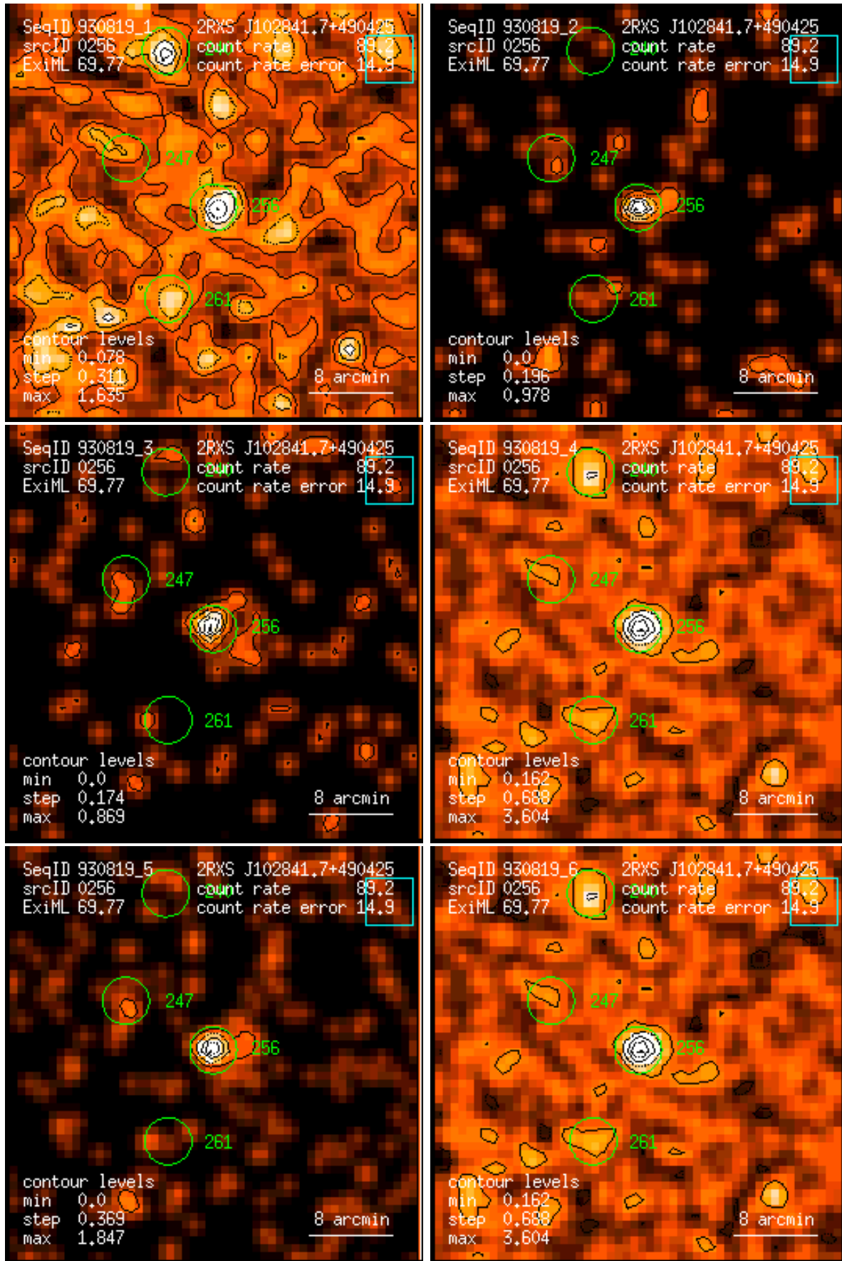
Figure 256: RASS 930819: detection 0256: band rate images, Gaussian filter: (1) PSPC channels 11 – 41, (2) 52 – 90, (3) 91 – 201, (4) 11 – 235, (5) 52 – 201, (6) 11 – 201. Broad band rates in counts/ks. Band rate contour levels in counts/ks/arcmin 2 .
