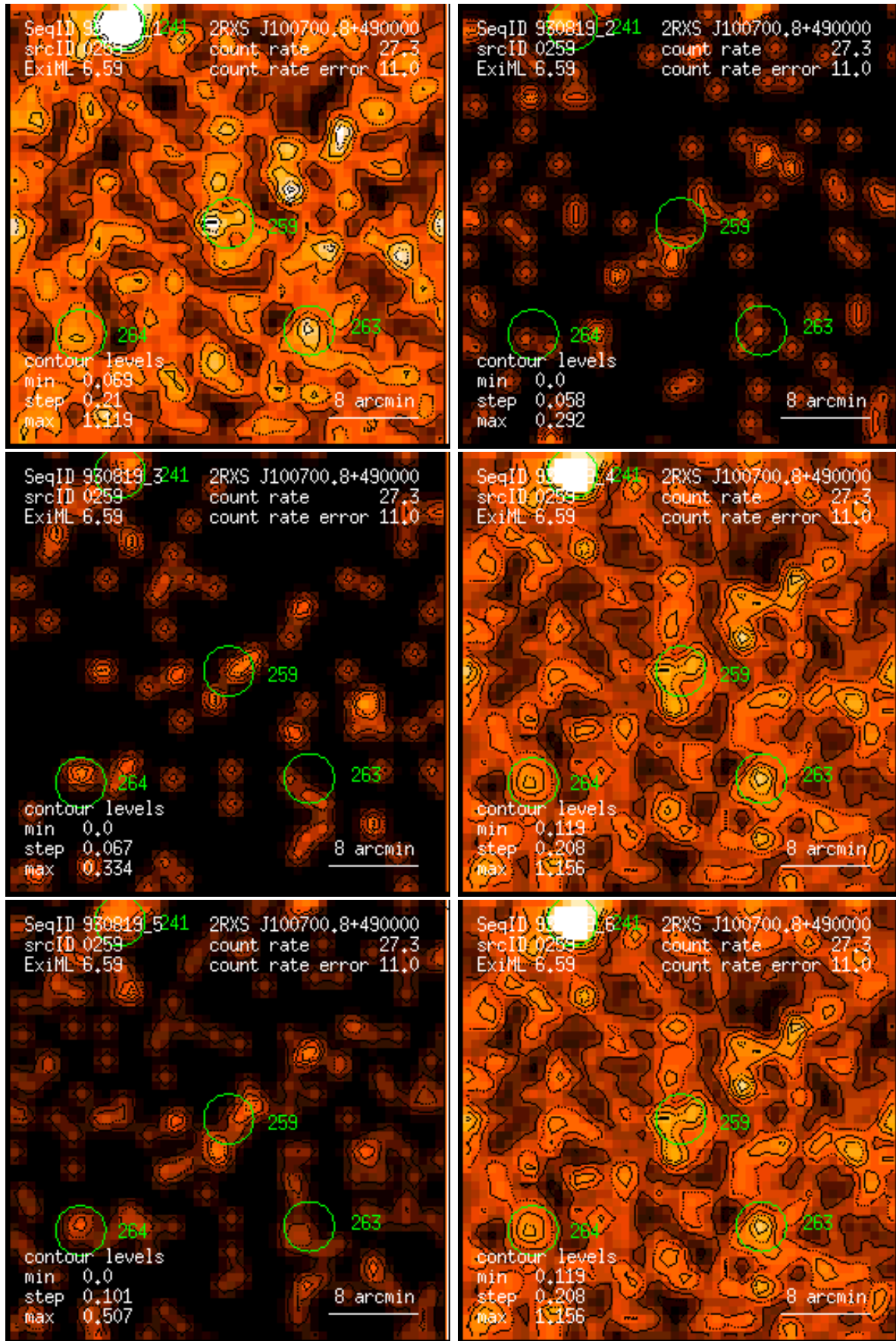
Figure 259: RASS 930819: detection 0259: band rate images, Gaussian filter: (1) PSPC channels 11 – 41, (2) 52 – 90, (3) 91 – 201, (4) 11 – 235, (5) 52 – 201, (6) 11 – 201. Broad band rates in counts/ks. Band rate contour levels in counts/ks/arcmin 2 .
