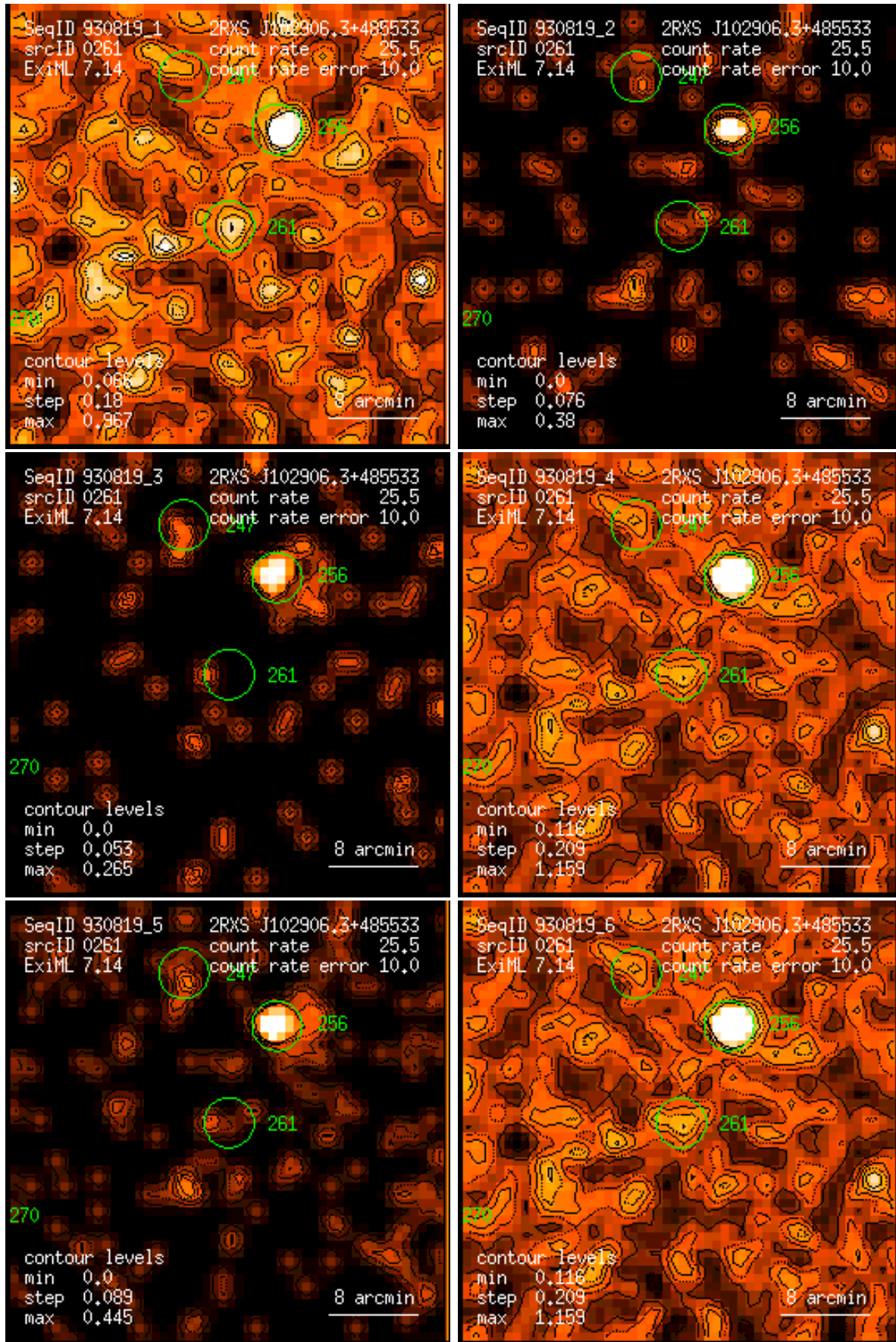
Figure 261: RASS 930819: detection 0261: band rate images, Gaussian filter: (1) PSPC channels 11 – 41, (2) 52 – 90, (3) 91 – 201, (4) 11 – 235, (5) 52 – 201, (6) 11 – 201. Broad band rates in counts/ks. Band rate contour levels in counts/ks/arcmin 2 .
