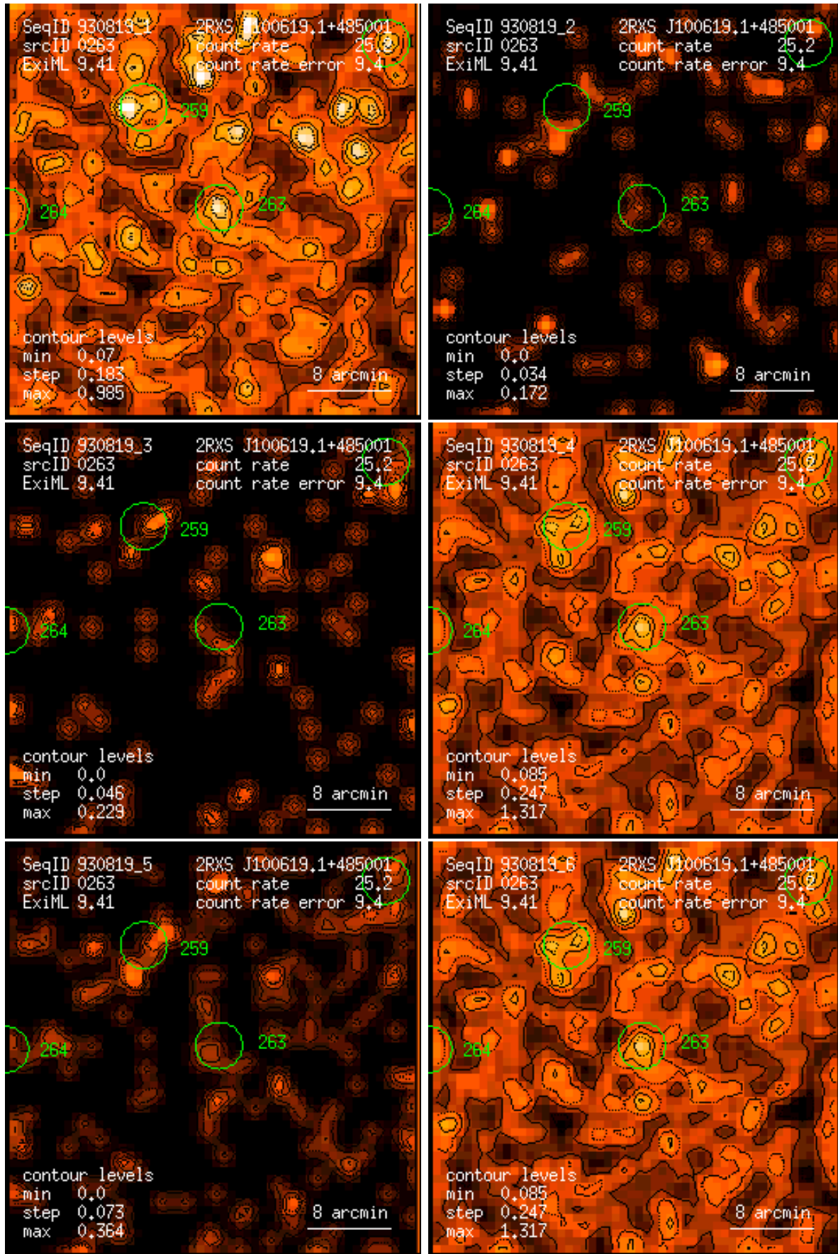
Figure 263: RASS 930819: detection 0263: band rate images, Gaussian filter: (1) PSPC channels 11 – 41, (2) 52 – 90, (3) 91 – 201, (4) 11 – 235, (5) 52 – 201, (6) 11 – 201. Broad band rates in counts/ks. Band rate contour levels in counts/ks/arcmin 2 .
