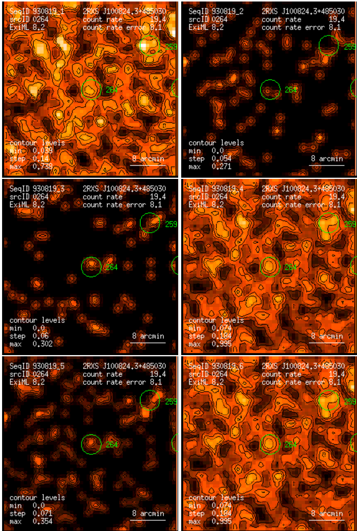
Figure 264: RASS 930819: detection 0264: band rate images, Gaussian filter: (1) PSPC channels 11 – 41, (2) 52 – 90, (3) 91 – 201, (4) 11 – 235, (5) 52 – 201, (6) 11 – 201. Broad band rates in counts/ks. Band rate contour levels in counts/ks/arcmin 2 .
