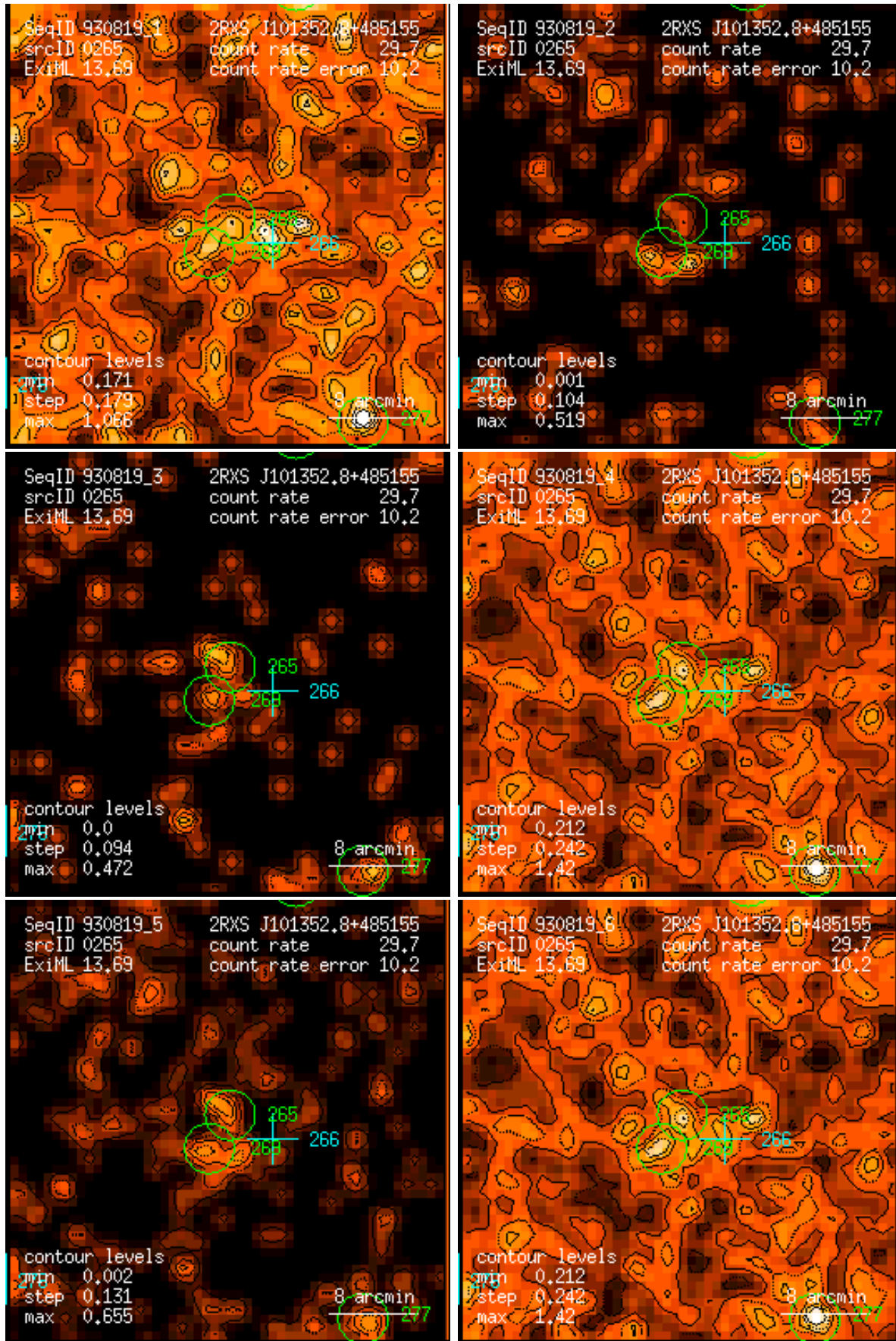
Figure 265: RASS 930819: detection 0265: band rate images, Gaussian filter: (1) PSPC channels 11 – 41, (2) 52 – 90, (3) 91 – 201, (4) 11 – 235, (5) 52 – 201, (6) 11 – 201. Broad band rates in counts/ks. Band rate contour levels in counts/ks/arcmin 2 .
