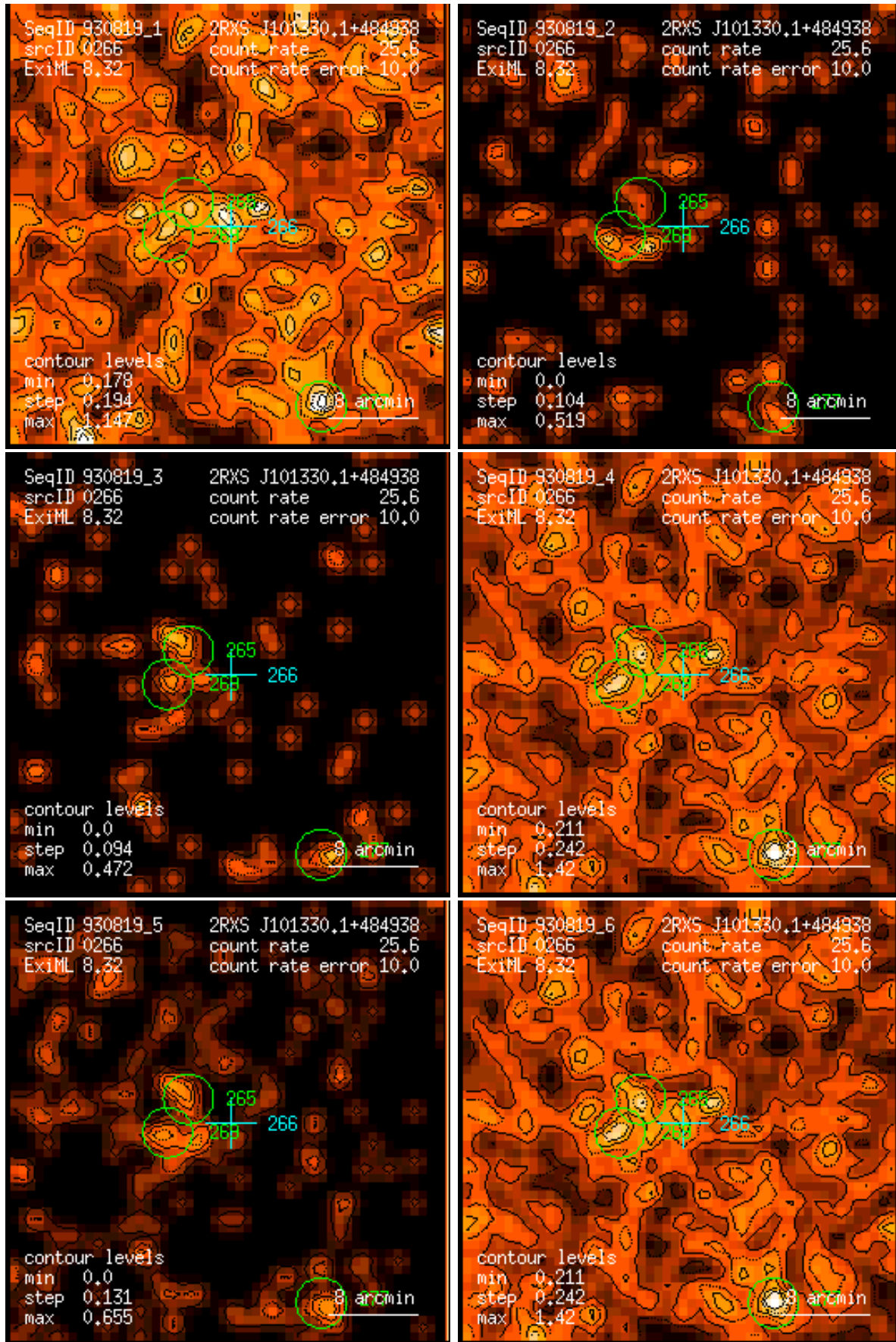
Figure 266: RASS 930819: detection 0266: band rate images, Gaussian filter: (1) PSPC channels 11 – 41, (2) 52 – 90, (3) 91 – 201, (4) 11 – 235, (5) 52 – 201, (6) 11 – 201. Broad band rates in counts/ks. Band rate contour levels in counts/ks/arcmin 2 .
