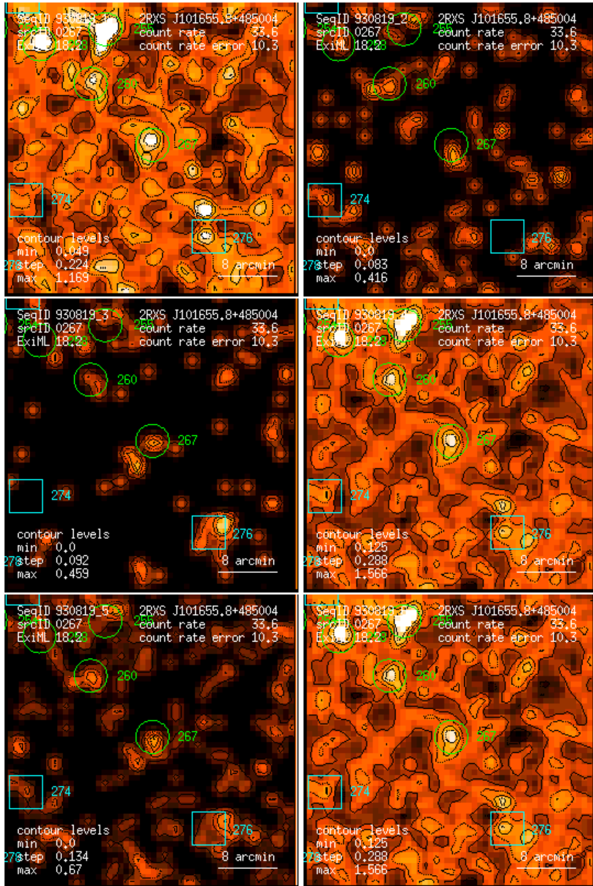
Figure 267: RASS 930819: detection 0267: band rate images, Gaussian filter: (1) PSPC channels 11 – 41, (2) 52 – 90, (3) 91 – 201, (4) 11 – 235, (5) 52 – 201, (6) 11 – 201. Broad band rates in counts/ks. Band rate contour levels in counts/ks/arcmin 2 .
