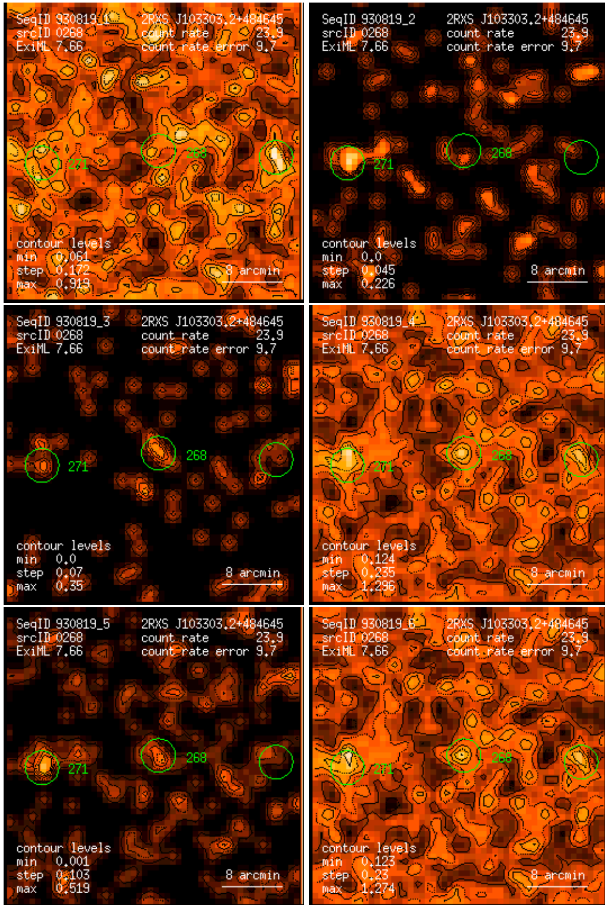
Figure 268: RASS 930819: detection 0268: band rate images, Gaussian filter: (1) PSPC channels 11 – 41, (2) 52 – 90, (3) 91 – 201, (4) 11 – 235, (5) 52 – 201, (6) 11 – 201. Broad band rates in counts/ks. Band rate contour levels in counts/ks/arcmin 2 .
