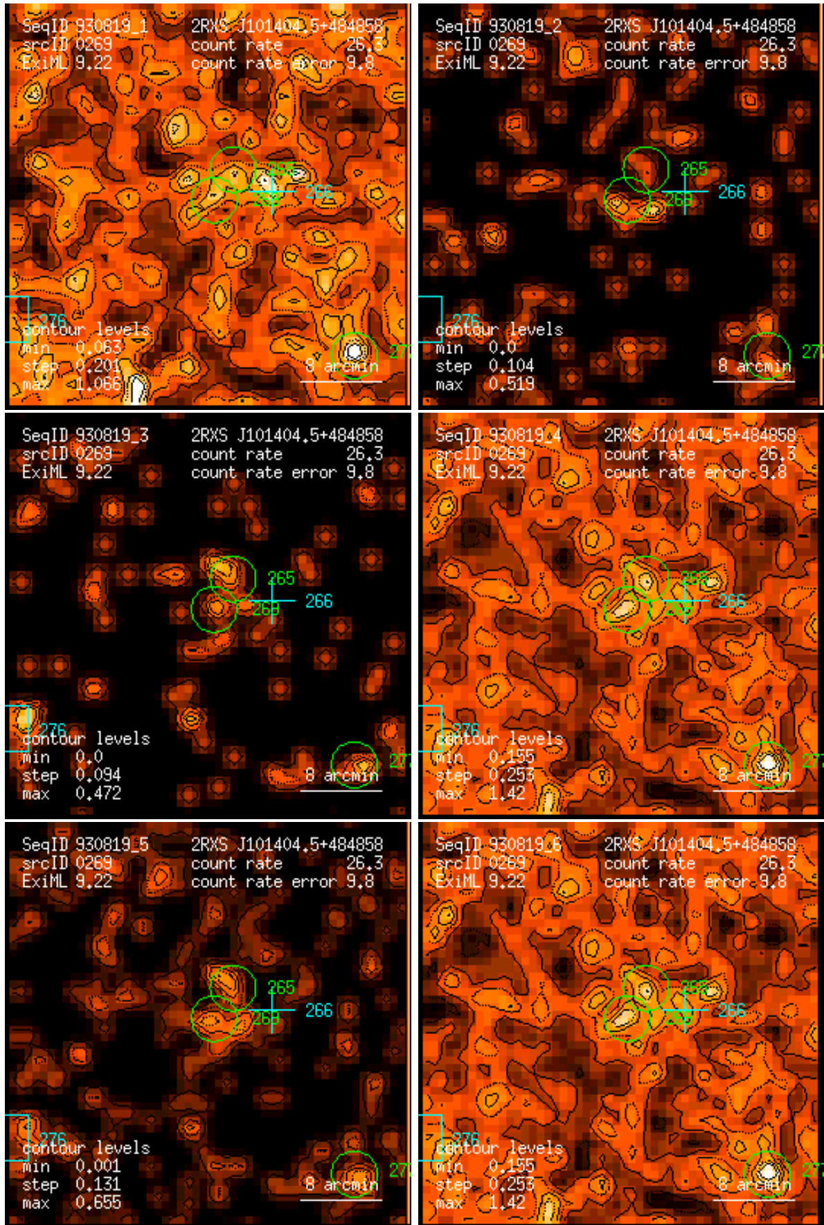
Figure 269: RASS 930819: detection 0269: band rate images, Gaussian filter: (1) PSPC channels 11 – 41, (2) 52 – 90, (3) 91 – 201, (4) 11 – 235, (5) 52 – 201, (6) 11 – 201. Broad band rates in counts/ks. Band rate contour levels in counts/ks/arcmin 2 .
