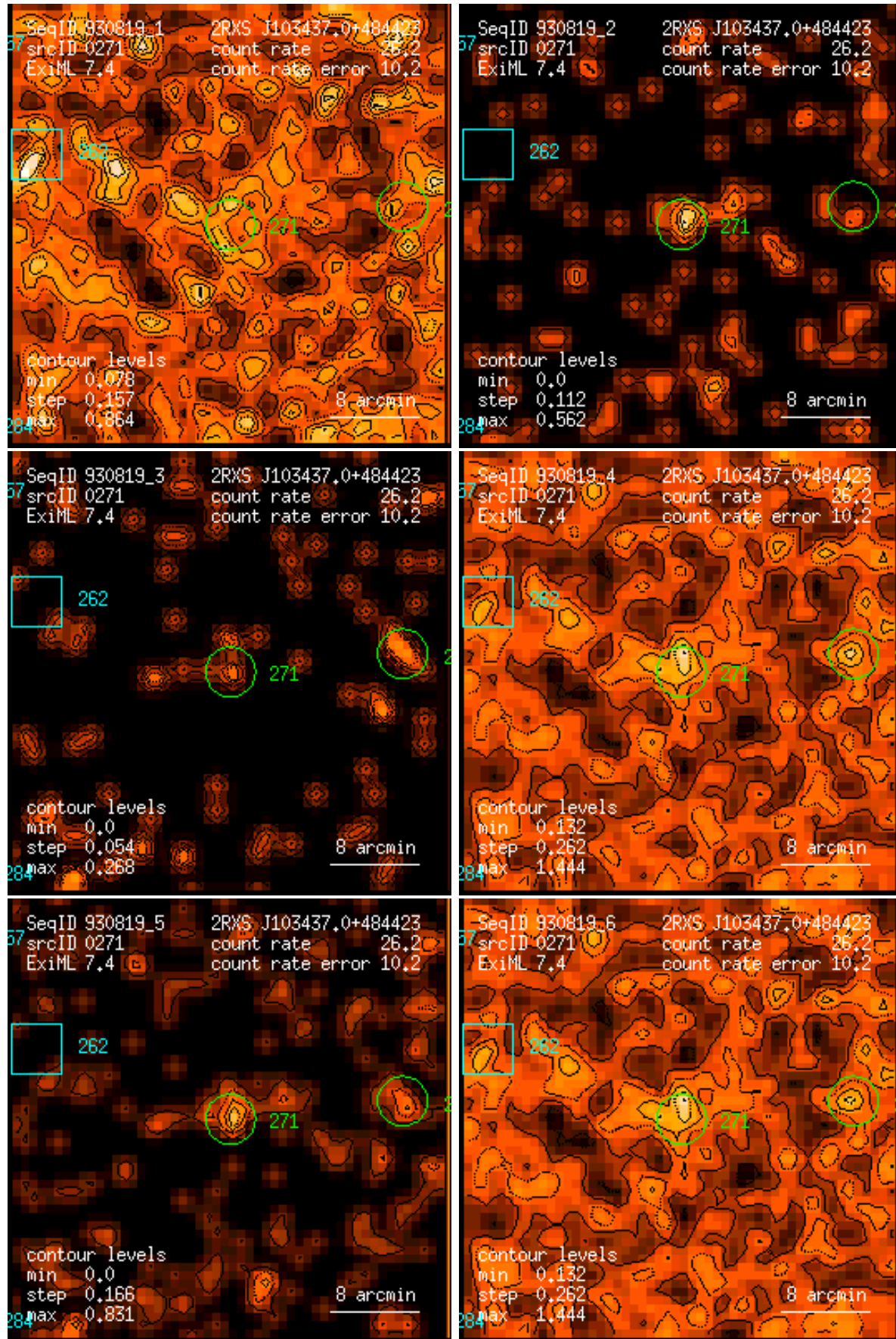
Figure 271: RASS 930819: detection 0271: band rate images, Gaussian filter: (1) PSPC channels 11 – 41, (2) 52 – 90, (3) 91 – 201, (4) 11 – 235, (5) 52 – 201, (6) 11 – 201. Broad band rates in counts/ks. Band rate contour levels in counts/ks/arcmin 2 .
