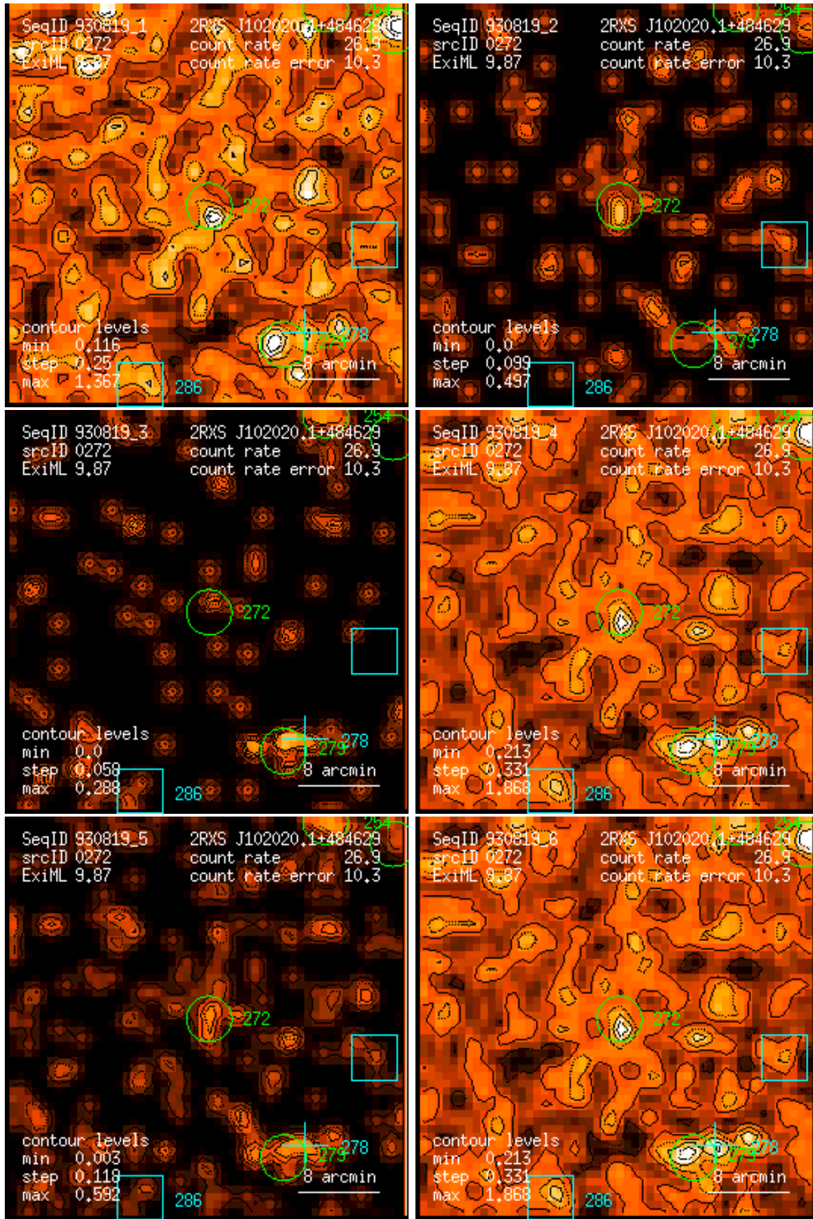
Figure 272: RASS 930819: detection 0272: band rate images, Gaussian filter: (1) PSPC channels 11 – 41, (2) 52 – 90, (3) 91 – 201, (4) 11 – 235, (5) 52 – 201, (6) 11 – 201. Broad band rates in counts/ks. Band rate contour levels in counts/ks/arcmin 2 .
