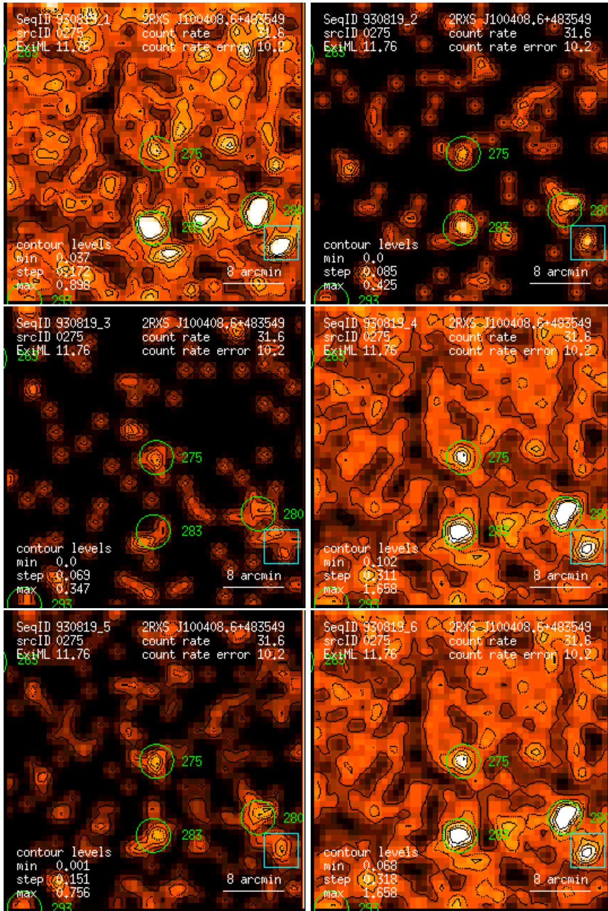
Figure 275: RASS 930819: detection 0275: band rate images, Gaussian filter: (1) PSPC channels 11 – 41, (2) 52 – 90, (3) 91 – 201, (4) 11 – 235, (5) 52 – 201, (6) 11 – 201. Broad band rates in counts/ks. Band rate contour levels in counts/ks/arcmin 2 .
