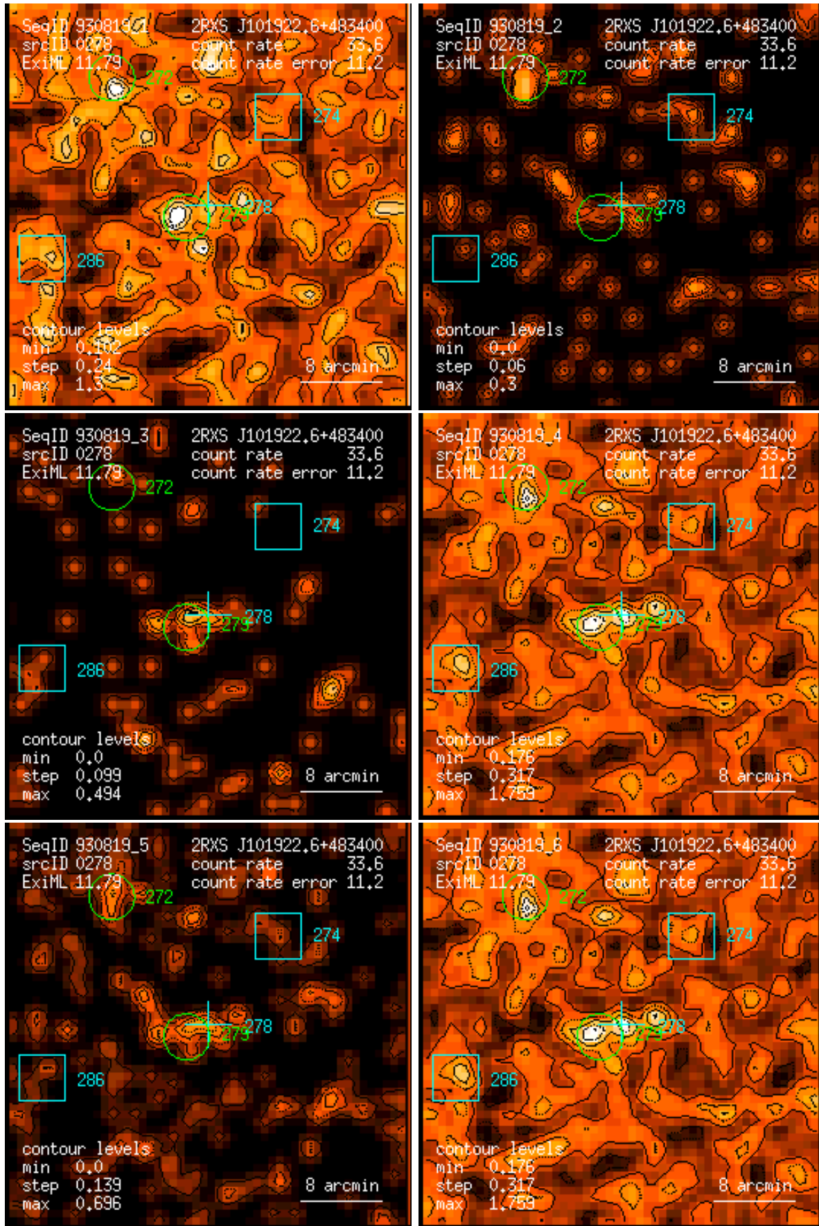
Figure 278: RASS 930819: detection 0278: band rate images, Gaussian filter: (1) PSPC channels 11 – 41, (2) 52 – 90, (3) 91 – 201, (4) 11 – 235, (5) 52 – 201, (6) 11 – 201. Broad band rates in counts/ks. Band rate contour levels in counts/ks/arcmin 2 .
