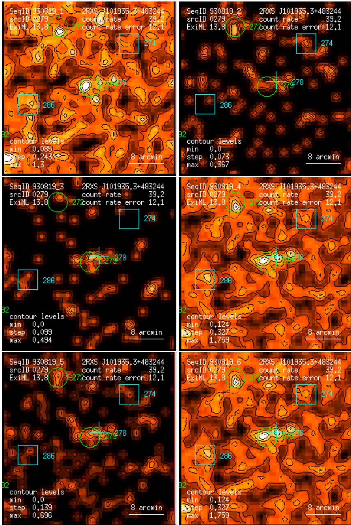
Figure 279: RASS 930819: detection 0279: band rate images, Gaussian filter: (1) PSPC channels 11 – 41, (2) 52 – 90, (3) 91 – 201, (4) 11 – 235, (5) 52 – 201, (6) 11 – 201. Broad band rates in counts/ks. Band rate contour levels in counts/ks/arcmin 2 .
