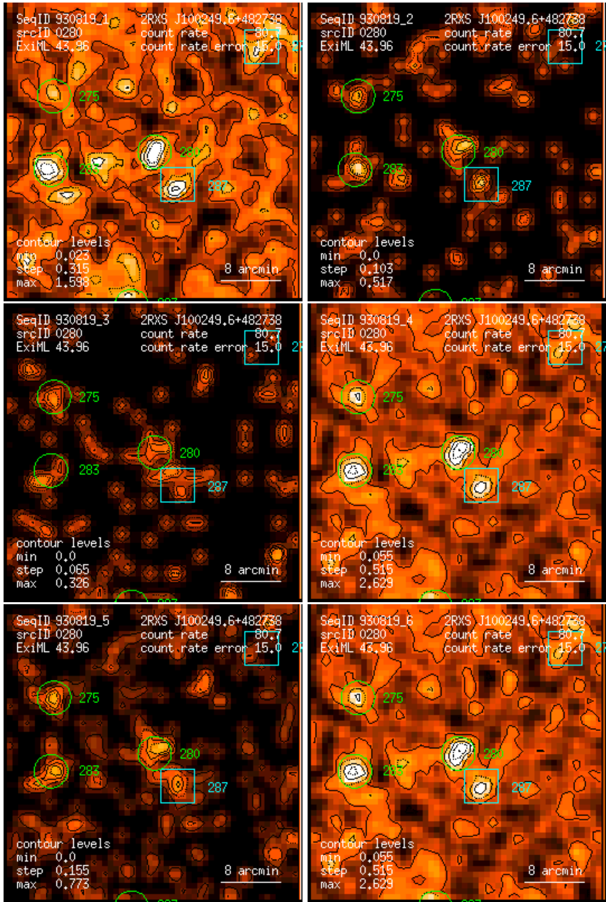
Figure 280: RASS 930819: detection 0280: band rate images, Gaussian filter: (1) PSPC channels 11 – 41, (2) 52 – 90, (3) 91 – 201, (4) 11 – 235, (5) 52 – 201, (6) 11 – 201. Broad band rates in counts/ks. Band rate contour levels in counts/ks/arcmin 2 .
