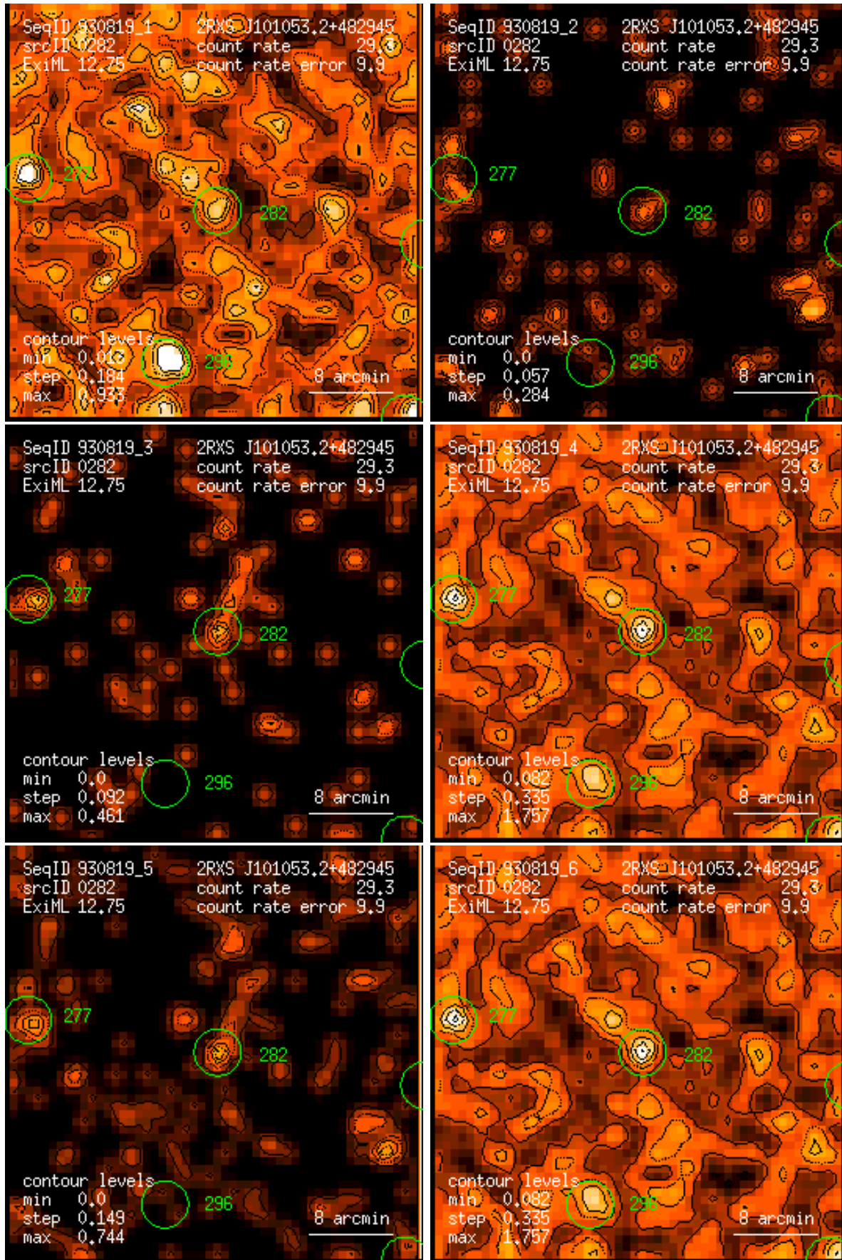
Figure 282: RASS 930819: detection 0282: band rate images, Gaussian filter: (1) PSPC channels 11 – 41, (2) 52 – 90, (3) 91 – 201, (4) 11 – 235, (5) 52 – 201, (6) 11 – 201. Broad band rates in counts/ks. Band rate contour levels in counts/ks/arcmin 2 .
