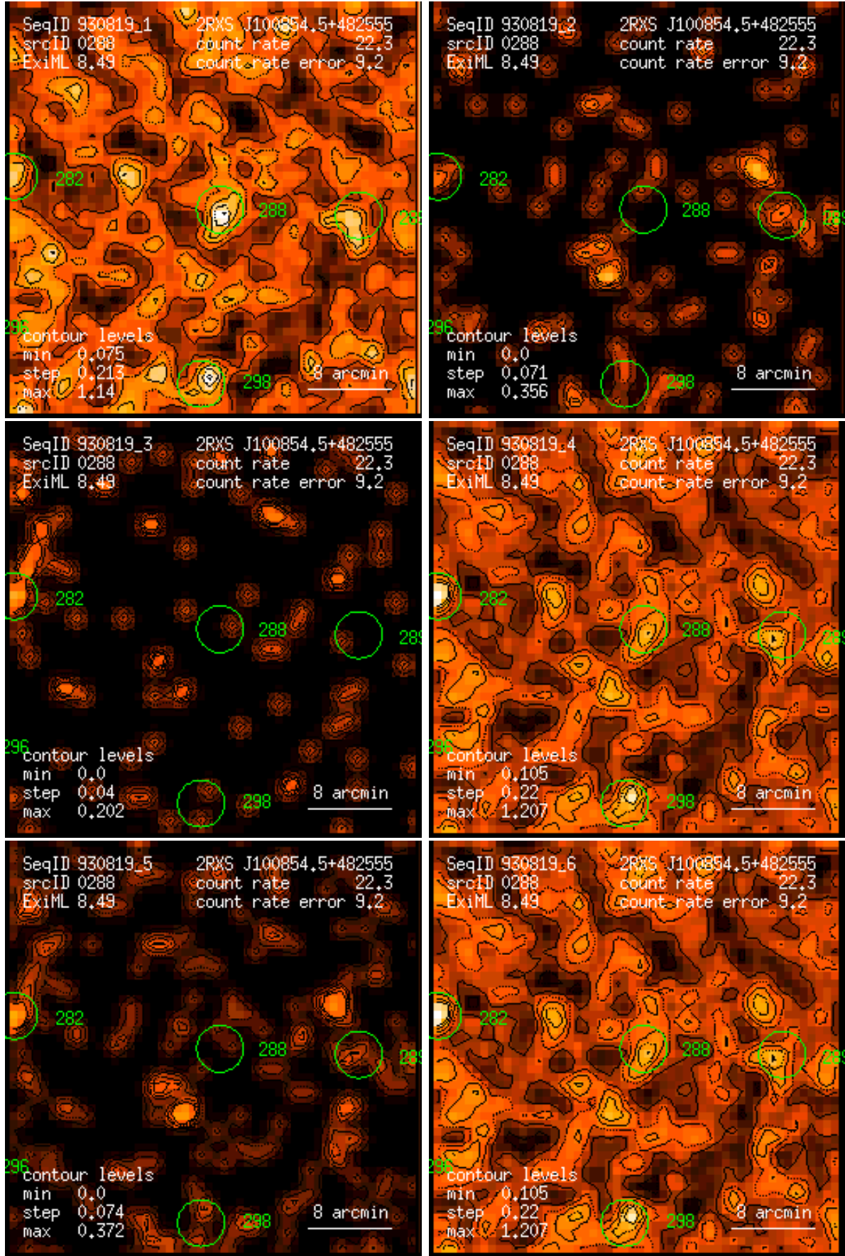
Figure 288: RASS 930819: detection 0288: band rate images, Gaussian filter: (1) PSPC channels 11 – 41, (2) 52 – 90, (3) 91 – 201, (4) 11 – 235, (5) 52 – 201, (6) 11 – 201. Broad band rates in counts/ks. Band rate contour levels in counts/ks/arcmin 2 .
