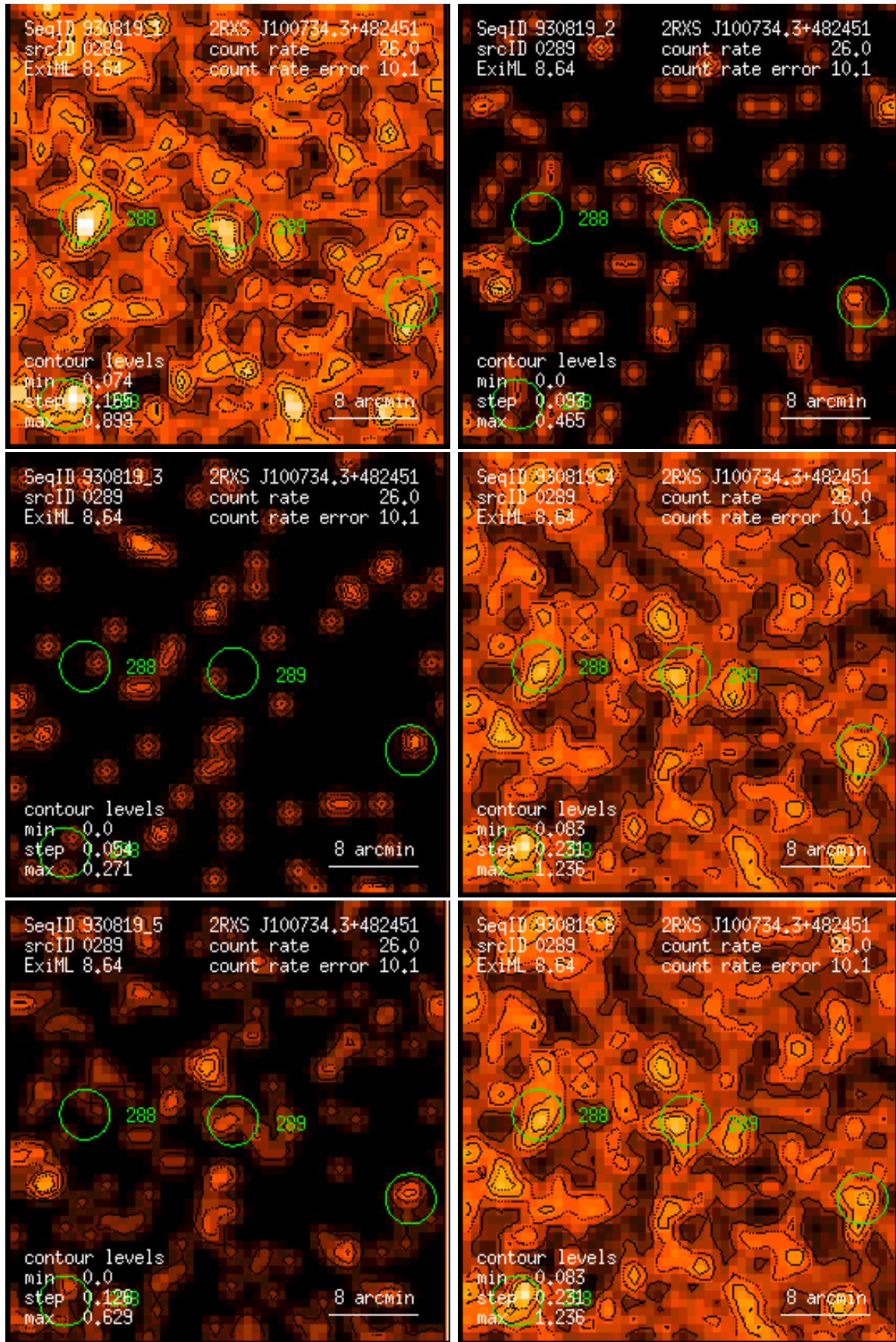
Figure 289: RASS 930819: detection 0289: band rate images, Gaussian filter: (1) PSPC channels 11 – 41, (2) 52 – 90, (3) 91 – 201, (4) 11 – 235, (5) 52 – 201, (6) 11 – 201. Broad band rates in counts/ks. Band rate contour levels in counts/ks/arcmin 2 .
