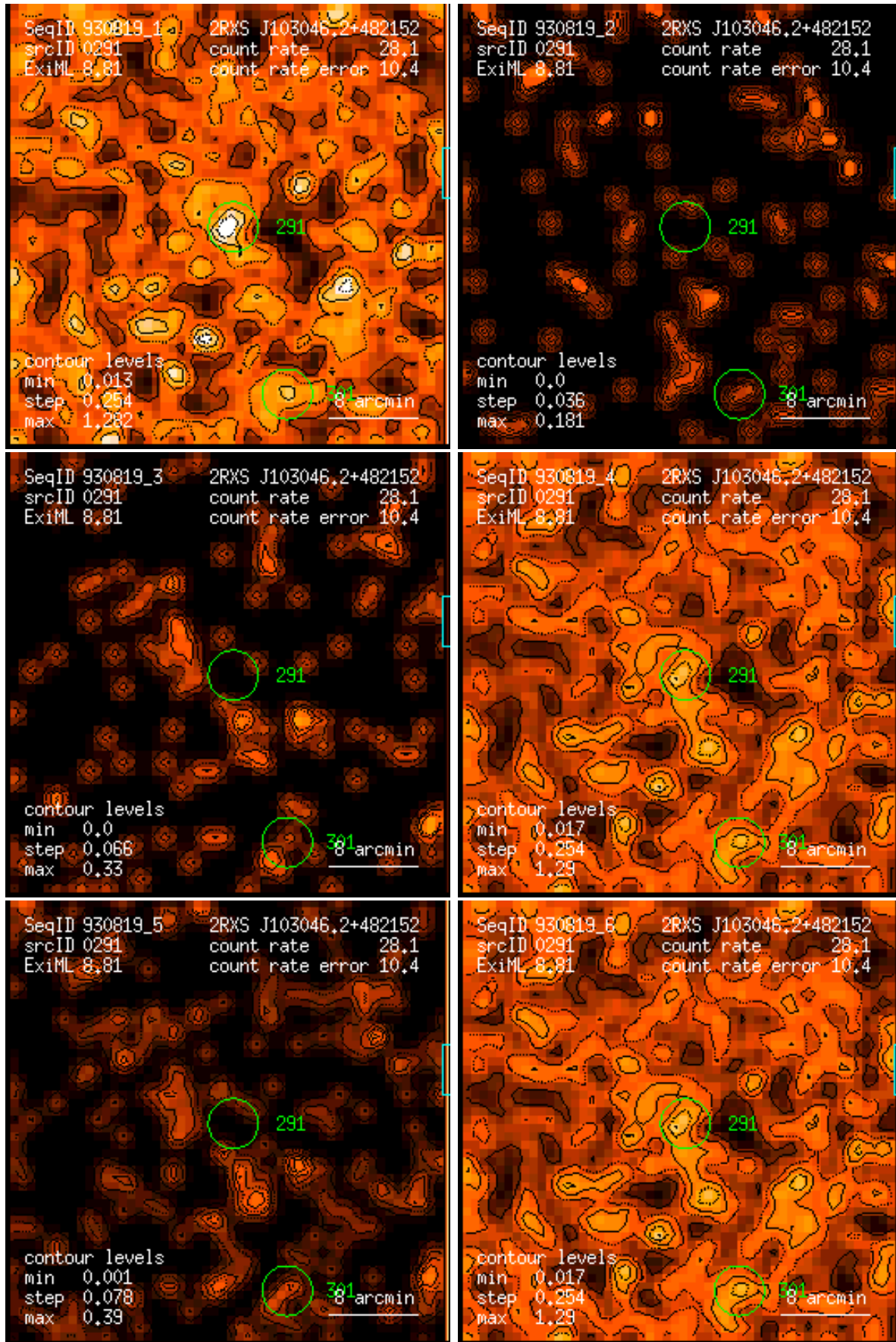
Figure 291: RASS 930819: detection 0291: band rate images, Gaussian filter: (1) PSPC channels 11 – 41, (2) 52 – 90, (3) 91 – 201, (4) 11 – 235, (5) 52 – 201, (6) 11 – 201. Broad band rates in counts/ks. Band rate contour levels in counts/ks/arcmin 2 .
