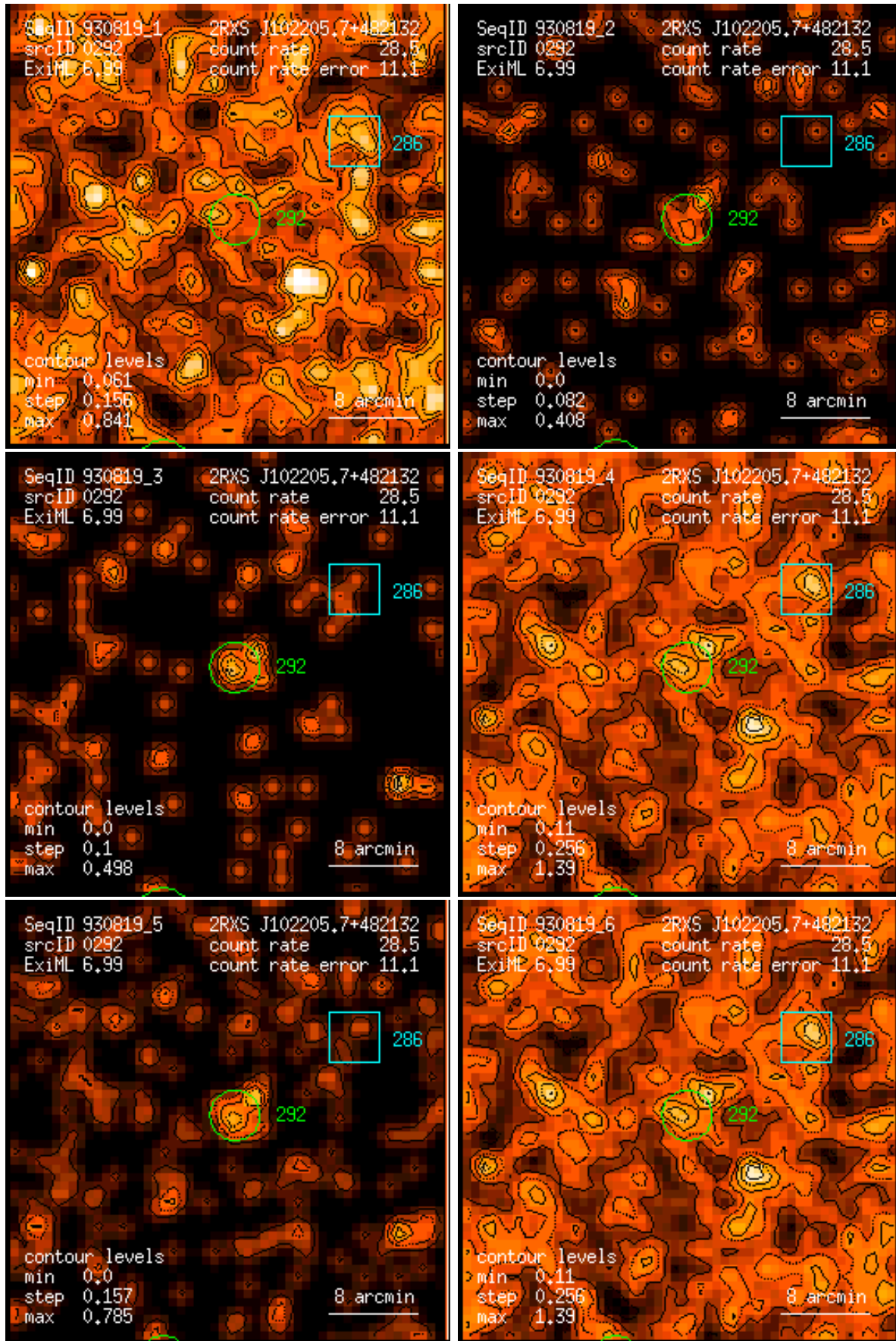
Figure 292: RASS 930819: detection 0292: band rate images, Gaussian filter: (1) PSPC channels 11 – 41, (2) 52 – 90, (3) 91 – 201, (4) 11 – 235, (5) 52 – 201, (6) 11 – 201. Broad band rates in counts/ks. Band rate contour levels in counts/ks/arcmin 2 .
