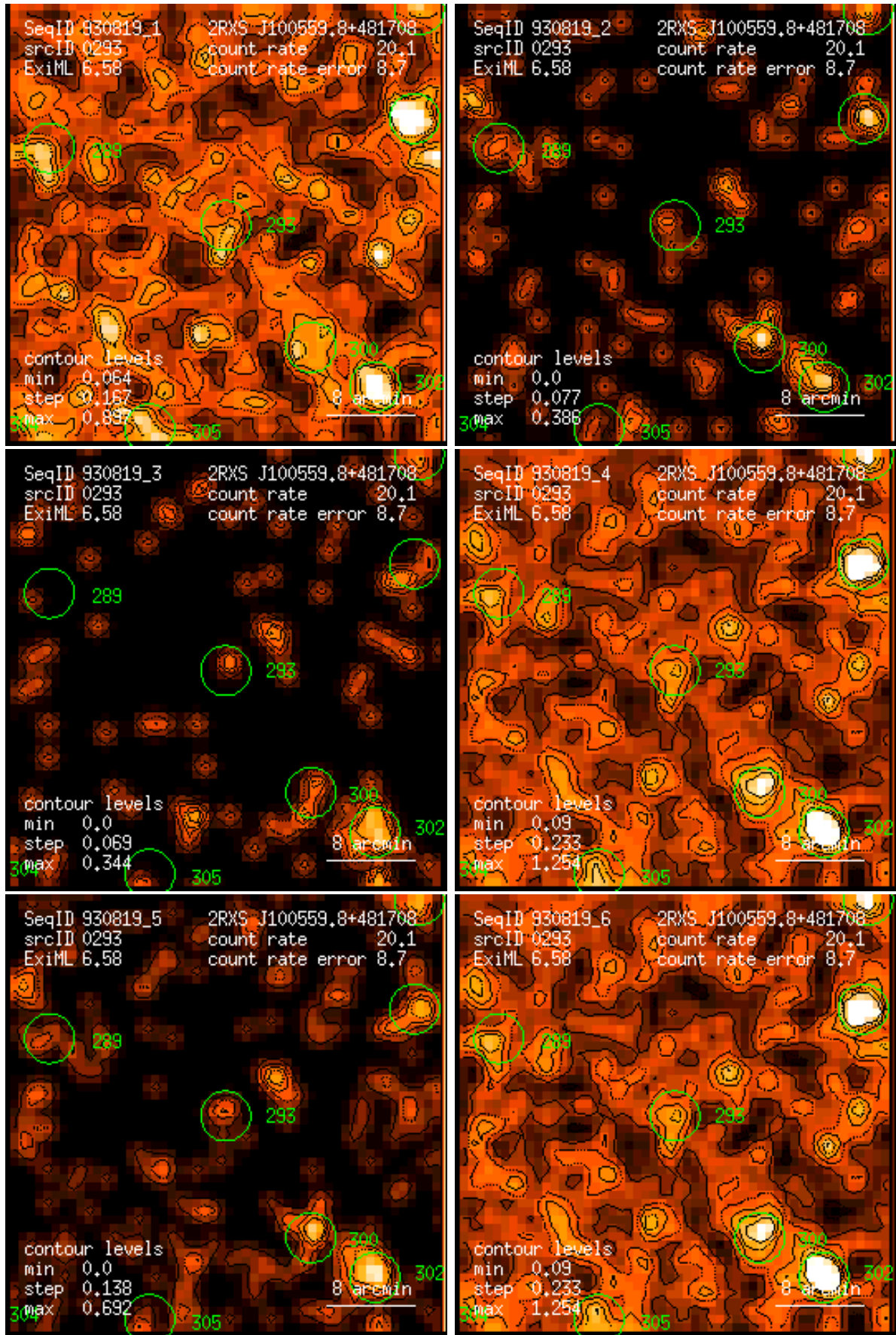
Figure 293: RASS 930819: detection 0293: band rate images, Gaussian filter: (1) PSPC channels 11 – 41, (2) 52 – 90, (3) 91 – 201, (4) 11 – 235, (5) 52 – 201, (6) 11 – 201. Broad band rates in counts/ks. Band rate contour levels in counts/ks/arcmin 2 .
