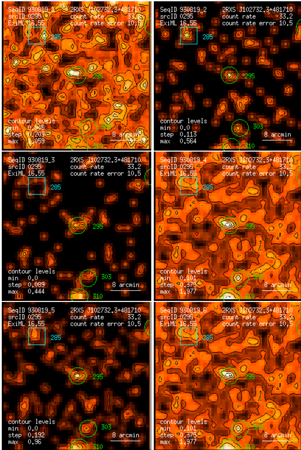
Figure 295: RASS 930819: detection 0295: band rate images, Gaussian filter: (1) PSPC channels 11 – 41, (2) 52 – 90, (3) 91 – 201, (4) 11 – 235, (5) 52 – 201, (6) 11 – 201. Broad band rates in counts/ks. Band rate contour levels in counts/ks/arcmin 2 .
