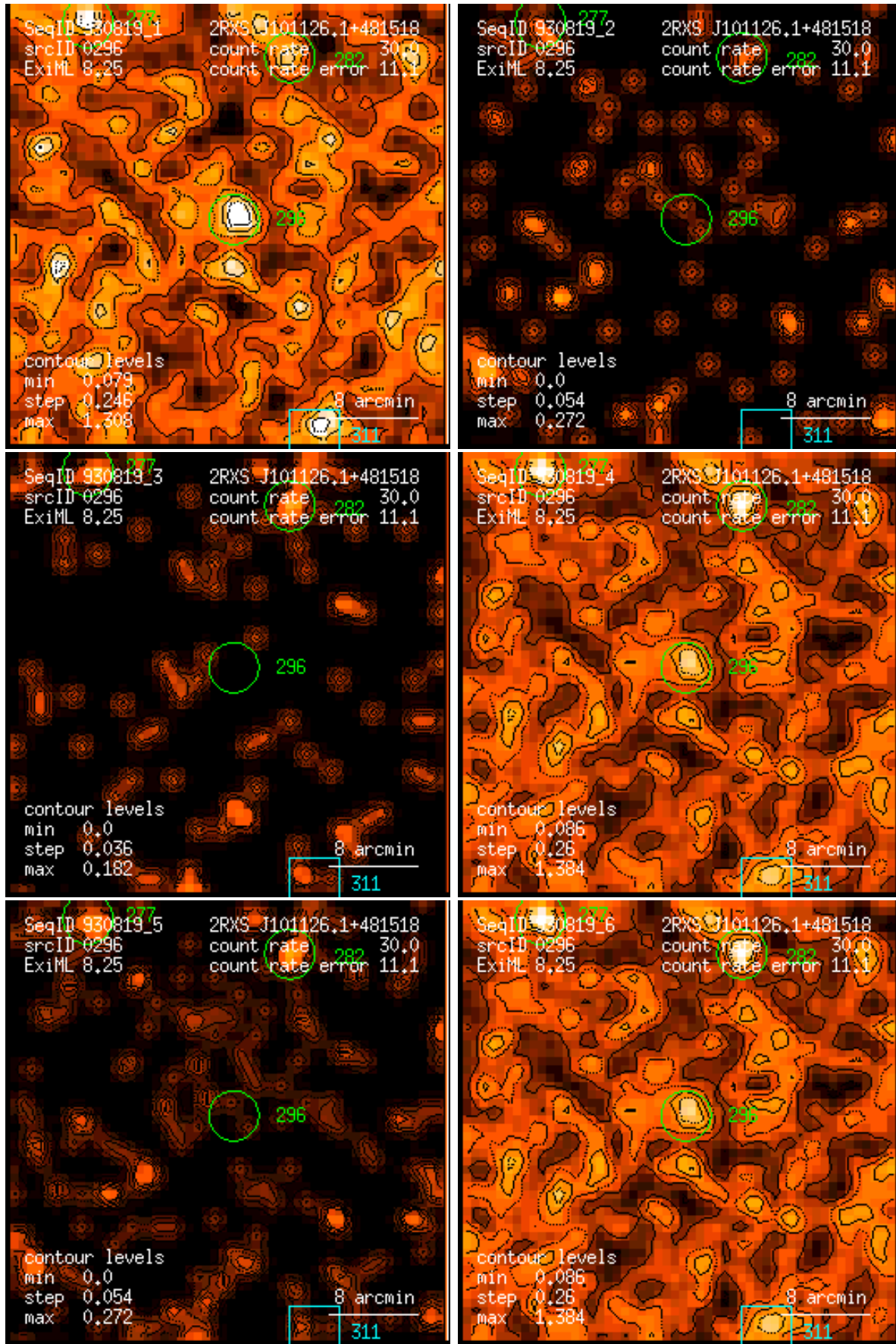
Figure 296: RASS 930819: detection 0296: band rate images, Gaussian filter: (1) PSPC channels 11 – 41, (2) 52 – 90, (3) 91 – 201, (4) 11 – 235, (5) 52 – 201, (6) 11 – 201. Broad band rates in counts/ks. Band rate contour levels in counts/ks/arcmin 2 .
